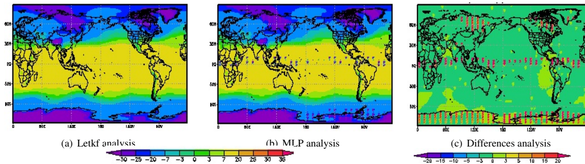
Figure 7 – Temperature ( ^{\circ}\text{C} ) Fields at layer 500 hPa to 03/01/2004 at 06 UTC. (a) LETKF analysis (b) MLP-DA analysis (c) differences between LETKF and MLP-DA analyses.
