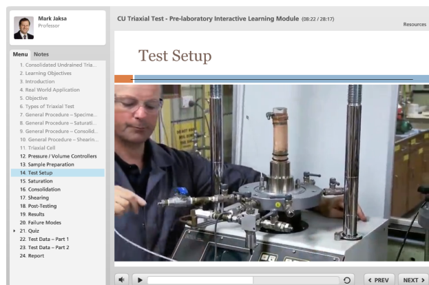
Figure 4. Video footage with narration explaining the setup of a triaxial test sample.
