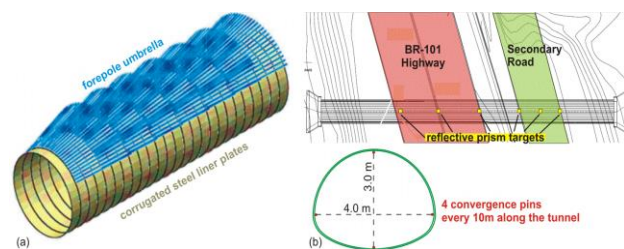
Figure 3. a) Auxiliary supporting means; b) convergence monitoring.
