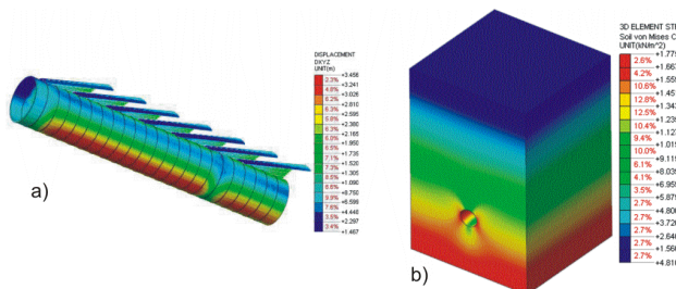
Figure 10. FE Analysis: a) stresses and axial forces – ULS; b) displacements – SLS.
