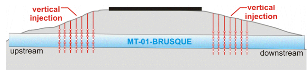
Figure 7. Grouting through multiple vertical injection pipes.
