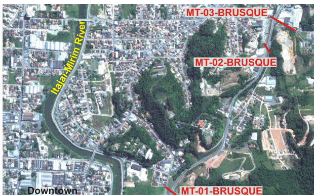
Figure 4. The 3 drainage microtunnels beneath a main road in Brusque.
