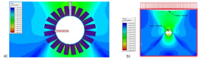
Figure 6. FE Analysis: a) stresses and axial forces – ULS; b) displacements – SLS.
