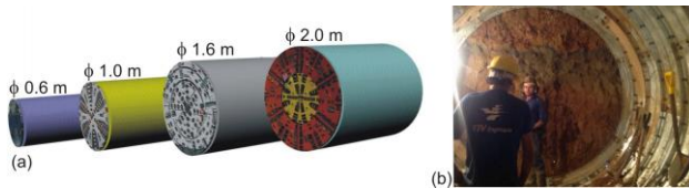
Figure 1. a) Microtunneling machines; b) hand digging.
