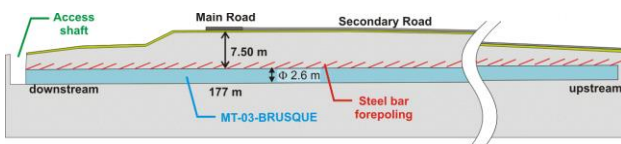
Figure 11. Microtunnel MT-03-Brusque basic plan.
