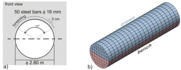
Figure 12. MT-03-Brusque: a) steel bar forepoling; b) partial face excavation.
