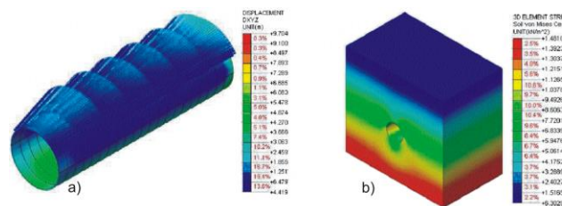
Figure 13. FE Analysis: a) stresses and axial forces – ULS; b) displacements – SLS.
