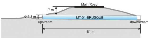
Figure 5. Microtunnel MT-01-Brusque basic plan.
