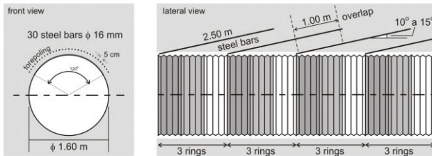
Figure 9. Steel bar forepoling for microtunnel MT-02-Brusque.
