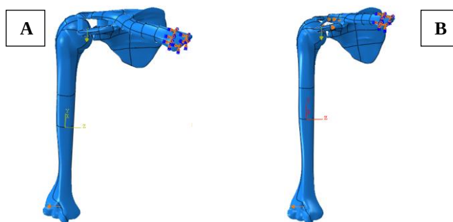
Figure 1: Boundary conditions applied to the models of surgical procedures. (A) Intact acromioclavicular joint, (B) Weaver-Dunn technique.
