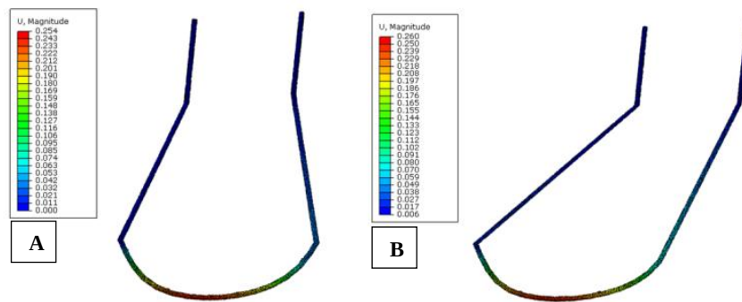
Figure 4: Gradients of resultant displacement [mm] for sutures. (A) Suture 1 (B) Suture 2.
