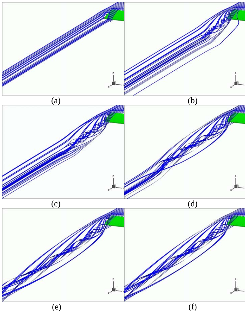
Figure 5: Evolution of streamlines over an NACA 0012 airfoil on times: (a) t=0.01s , (b) t=1.0s (c) t=1.5s (d) t=3.0s (e) t=5.0s (f) t=10.0s .
