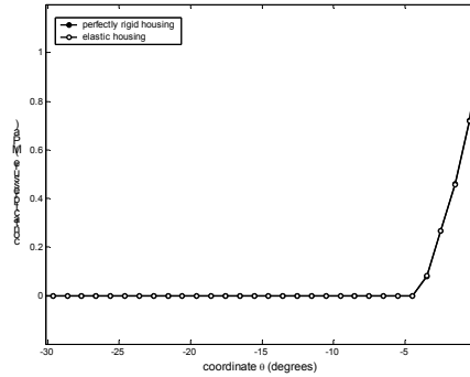
Figure 8: Contact pressure distribution at the interface between the insert bearing and the housing due to the bearing spread.
