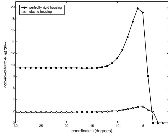
Figure 12: Distribution of radial reaction (contact pressure) on the insert due to the bearing crush.
