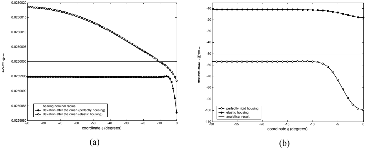
Figure 10: (a) Distribution of radial displacement and (b) hoop stress due to the bearing crush.
