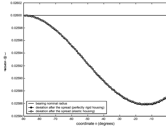
Figure 6: Distribution of radial displacement due to the bearing spread.
