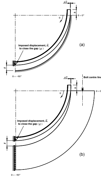
Figure 4: Configurations used for the analysis of the bearing spread: (a) perfectly rigid housing, and (b) elastic housing.
