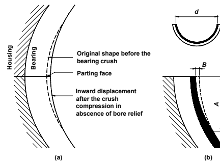
Figure 3: Bore relief. (a) Effect that would arise in absence of bore relief (for simplicity, no lining is shown in this figure); and (b) bore relief.
