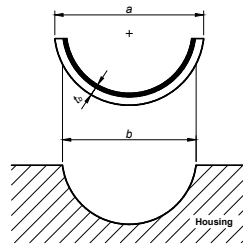
Figure 1: Bearing spread. The bearing diameter, a , is a trifle larger than the bore diameter b .
