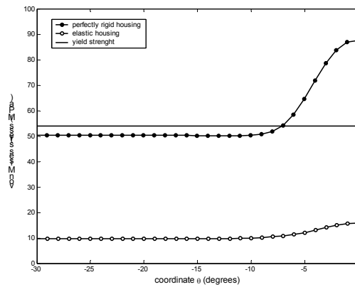
Figure 11: Distribution of equivalent (von Mises) stress at the surface of the bearing due to the bearing crush.
