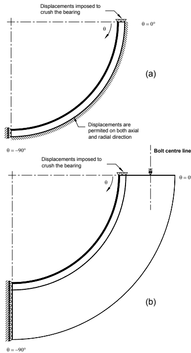
Figure 5: Configurations used for the analysis of the bearing crush: (a) perfectly rigid housing, and (b) elastic housing.
