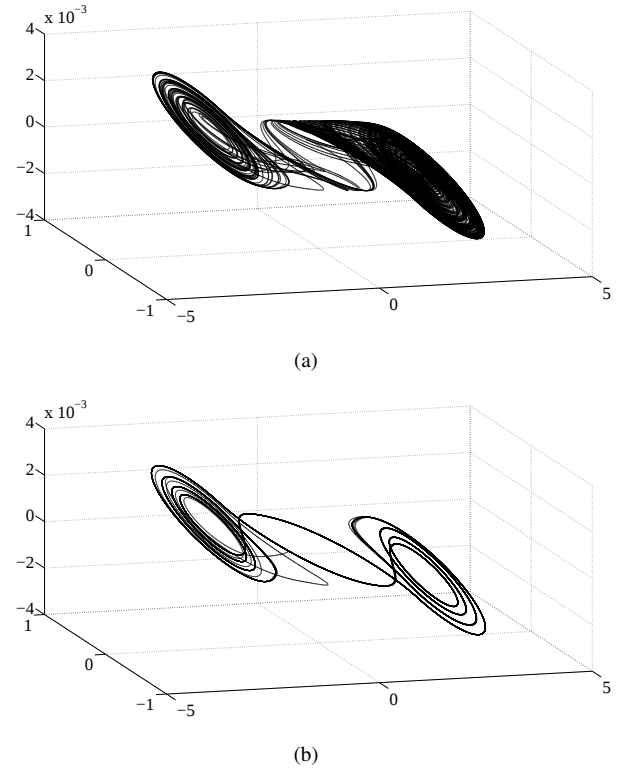
Figure 3: Scroll of Chua's circuit.
