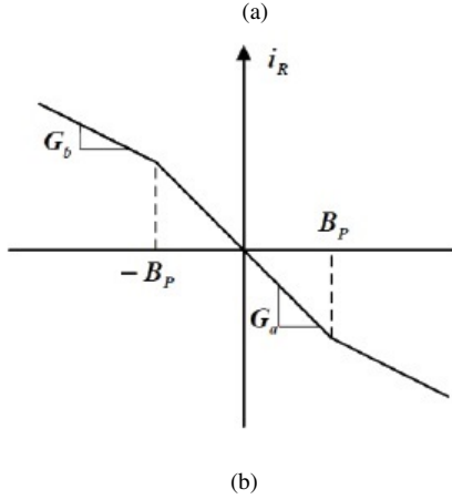
Figure 1: The Chua's circuit [1]. (a) the Chua' circuit and (b) curve of Chua diode (current-voltage characteristic).
