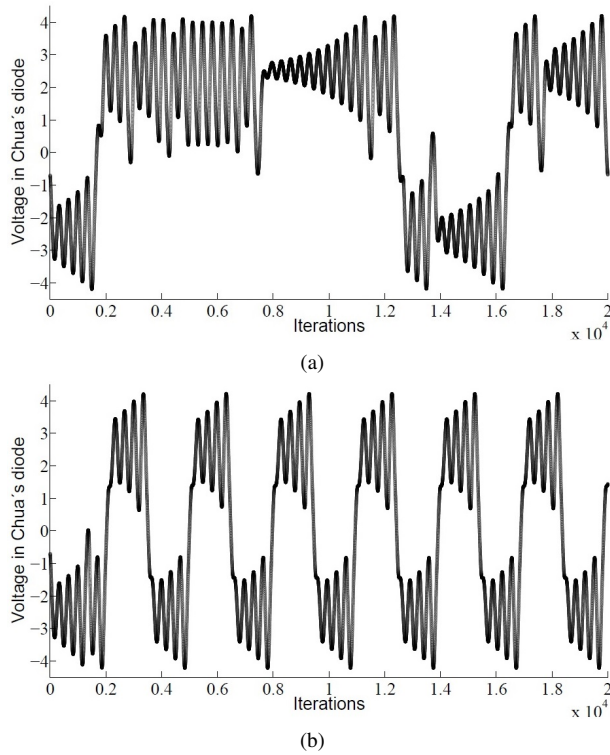
Figure 2: Voltage in Chua's diode.
