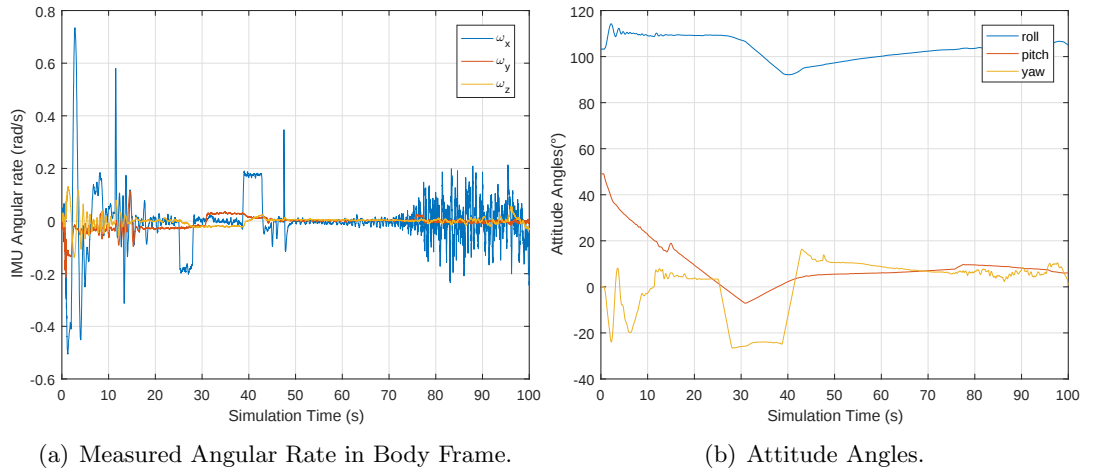
Figure 1: Attitude and angular rate.
