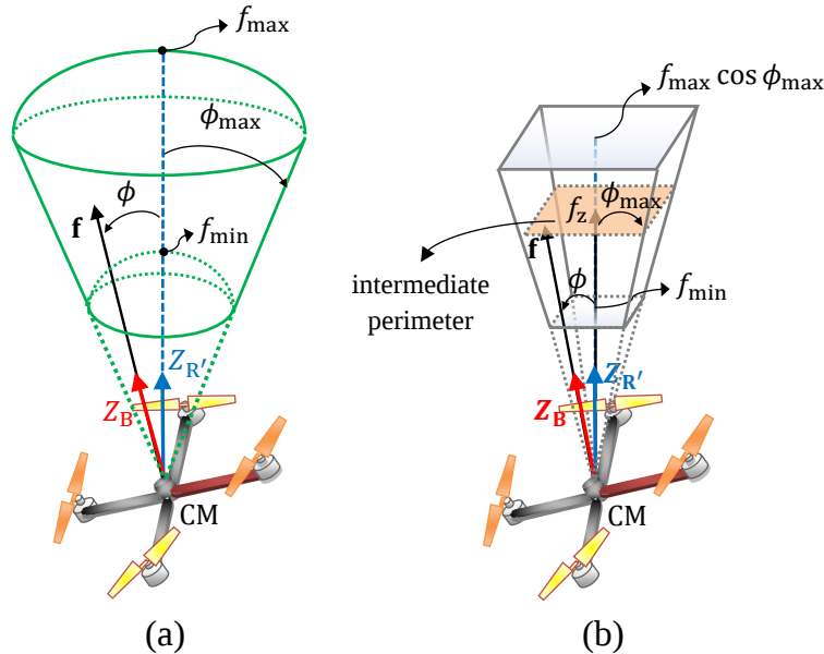
Figure 2: (a) Original constraints space; (b) Linearized constraints space.
