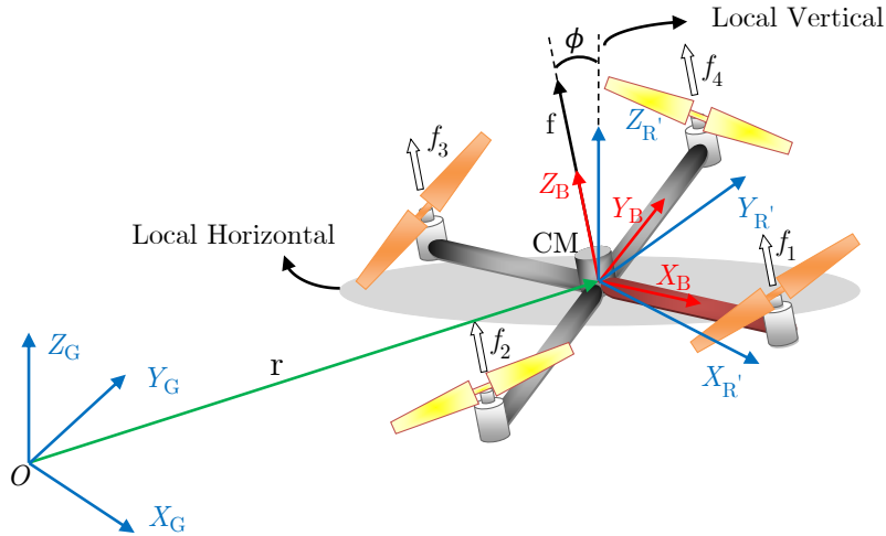
Figure 1: The Cartesian coordinate systems (CCS). S_B = \{X_B, Y_B, Z_B\} is the body CCS and S_G = \{X_G, Y_G, Z_G\} is the ground CCS.
