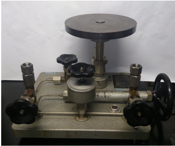
Figure 2: The VEB Gerätewerk pressure balance studied.
