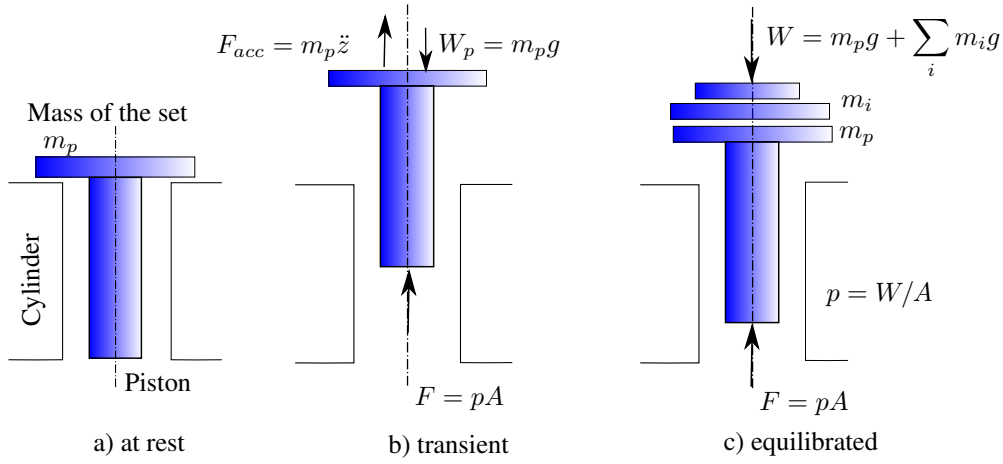
Figure 1: Pressure balance measuring principle: a) the balance is at rest, b) transient phase when the balance is put under pressure, c) disks of variable masses are put on the top of the balance as to find an equilibrated position.
