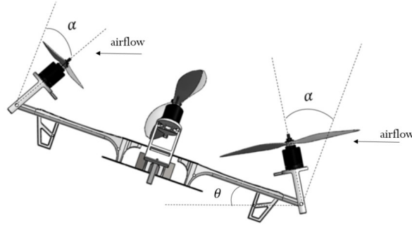
Figura 2: 2D visualization of a QTRH moving to the right (airflow to the left with respect to the hovercraft).
