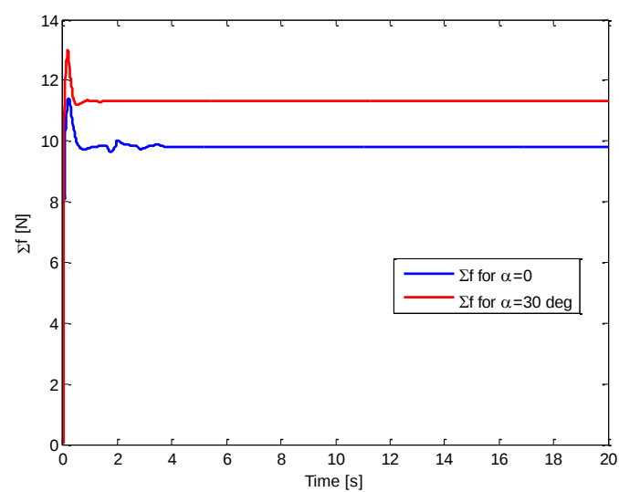
Figura 9: Sum of the thrust forces of each rotor on the simulation of task 2.
