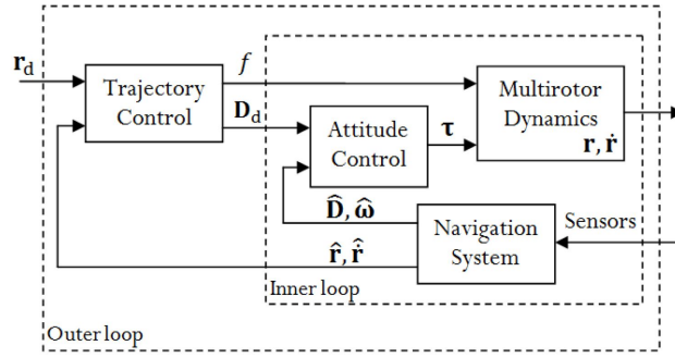
Figura 3: Schematic structure of a MAV control system.
