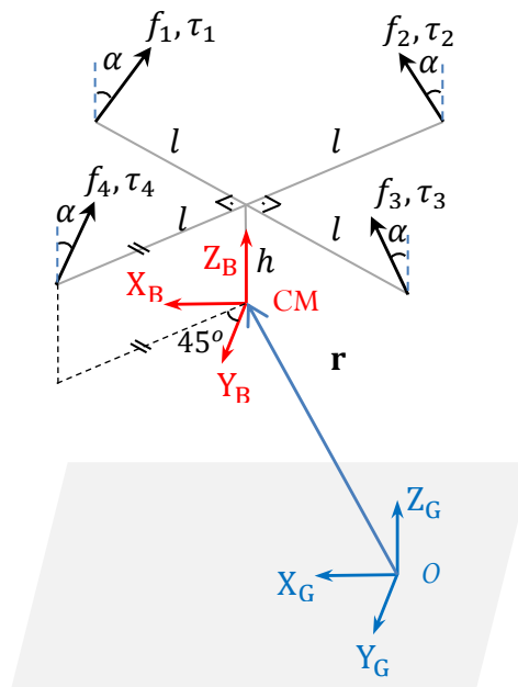
Figura 1: Schematic structure of the Quad Tilt Rotors Hovercraft.
