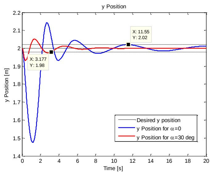
Figura 8: Position y from the results of the simulation of task 2.
