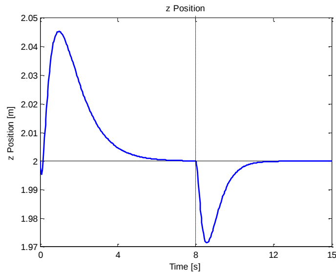
Figura 10: Z position of the MAV while the rotors are being tilted from 0 to 30 degrees at 0 seconds and from 30 degrees to 0 at 8 seconds.
