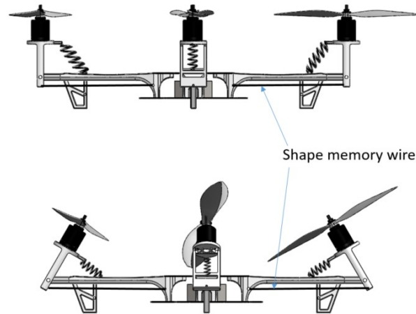
Figura 5: Side view of the QTRH with the rotors in the straight and tilted position.
