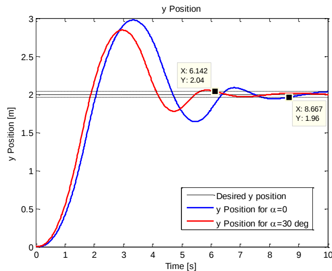
Figura 6: Results of the simulation of task 1.
