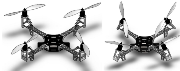
Figura 4: Isometric view of the QTRH with the rotors in the straight position (left) and in the tilted position (right).
