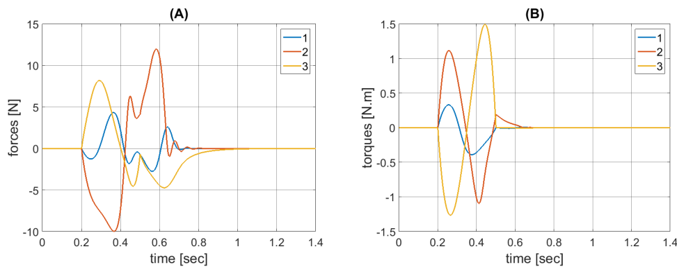
Figure 7: (A) Forces and (B) torques of the redundant robot
