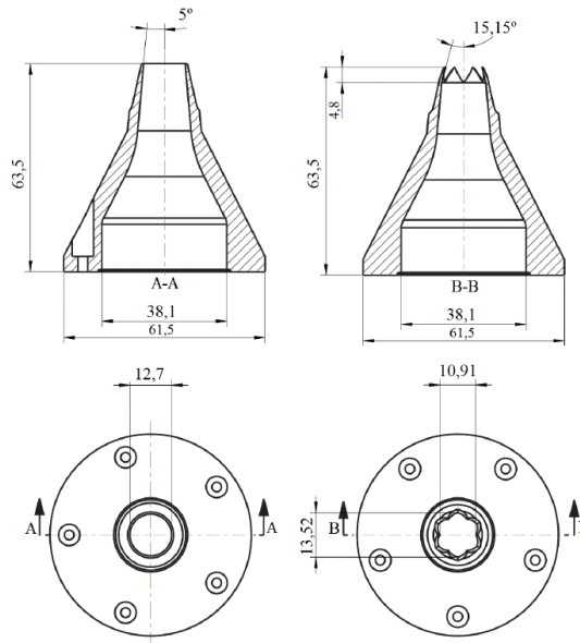
Figure 2: Nozzle geometry and dimensions.
