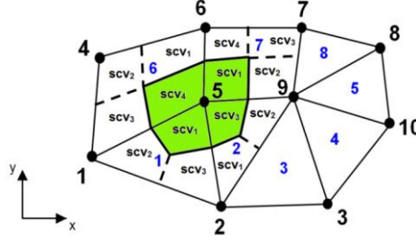
Figure 1. Illustration of a control-volume for the EbFVM approach.
