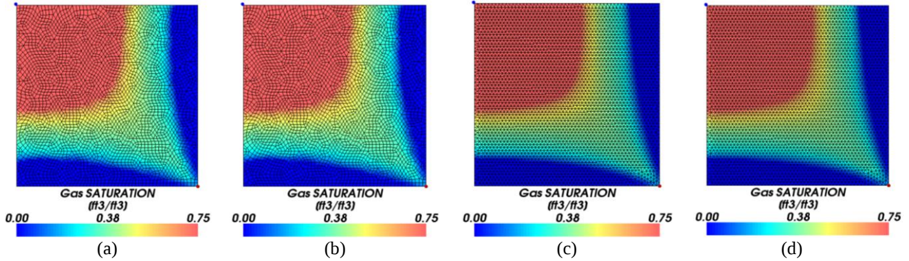
Figure 3. CO 2 rich phase at 500 days of simulation. a) IMPEC and b) IMPSAT, 3,387 vertices grid with 3,282 quadrilateral elements; c) IMPEC and d) IMPSAT, 3,329 vertices grid with 6,444 triangle elements
