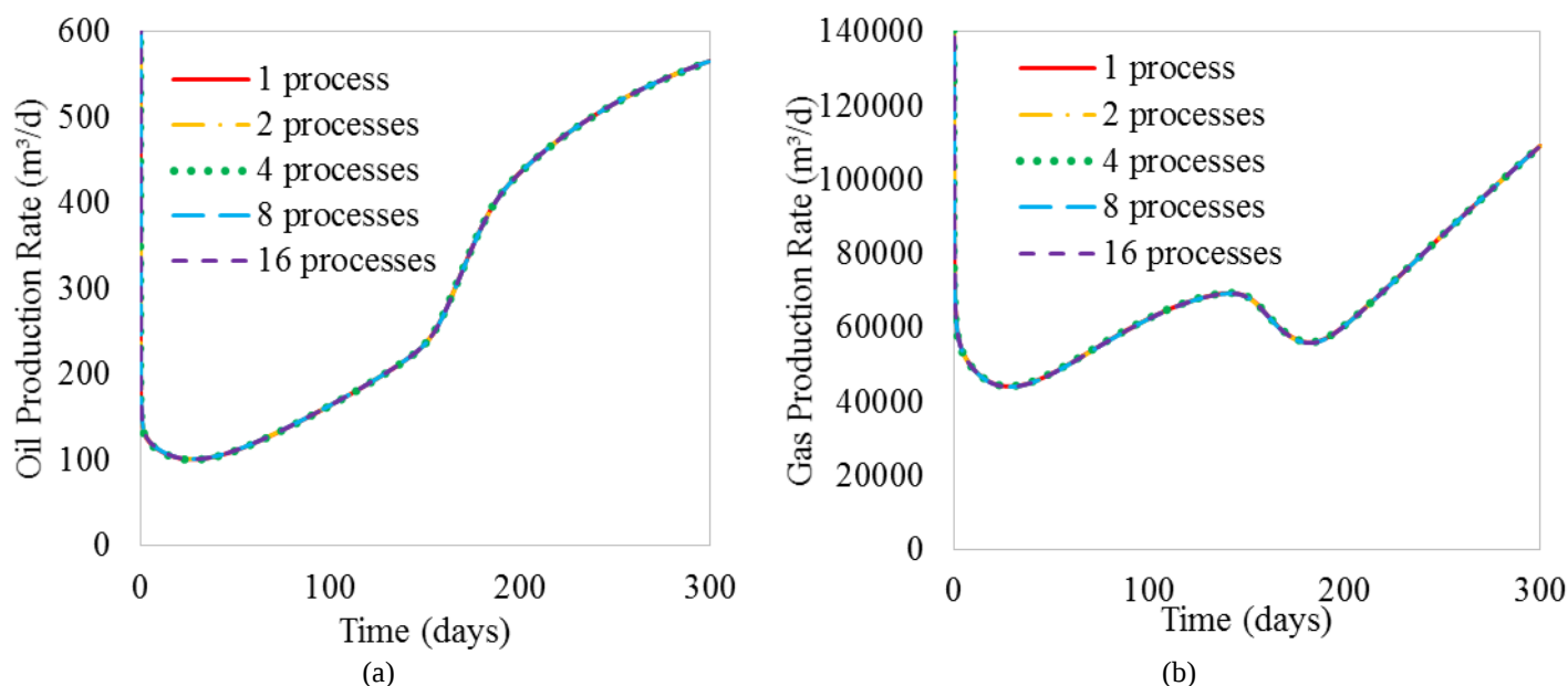
Figure 7. Standard volumetric rates for case 2. a) Oil production b) Gas production
