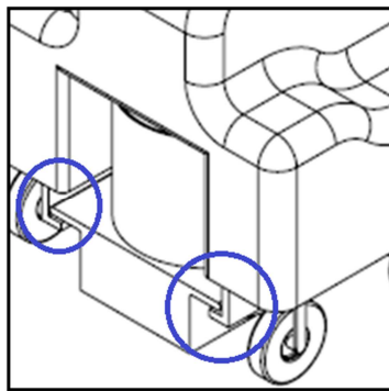
Figure 5. Coupling detail.
