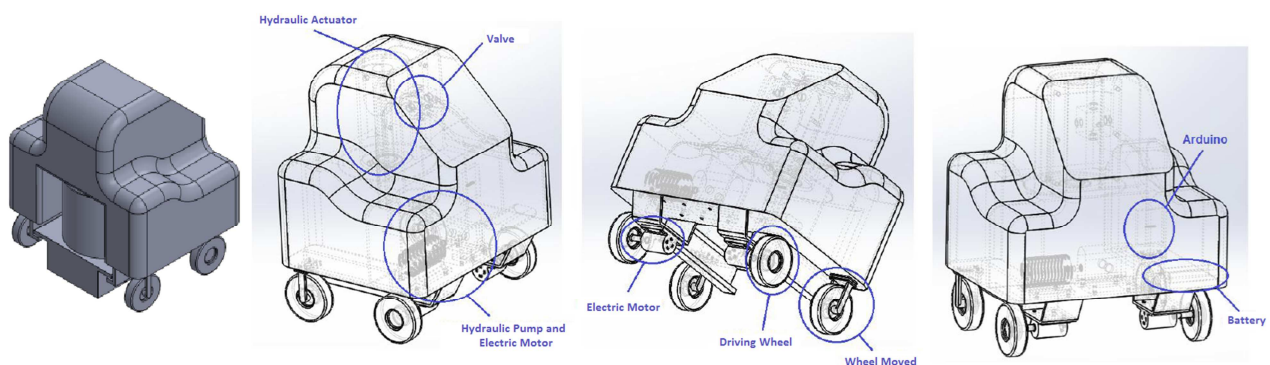
Figure 7. Modeling of the robot's system.
