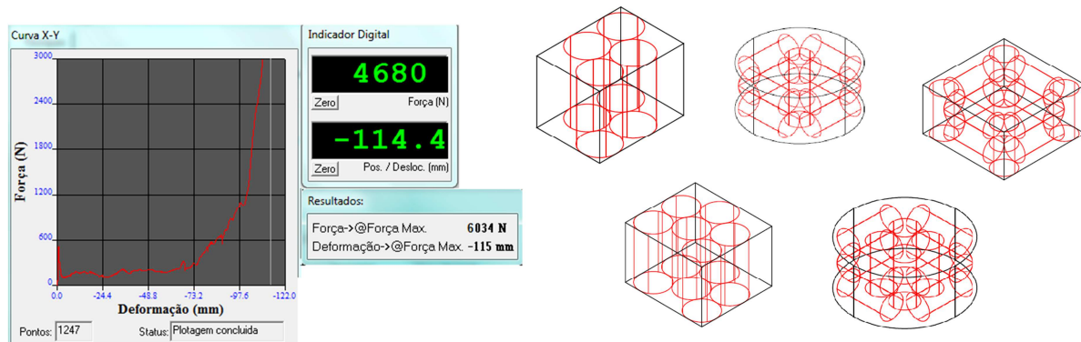
Figure 2. Force needed to compress a can and study of the trash can dimensions.
