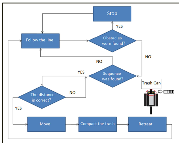
Figure 6. Flowchart of the robot's operations.
