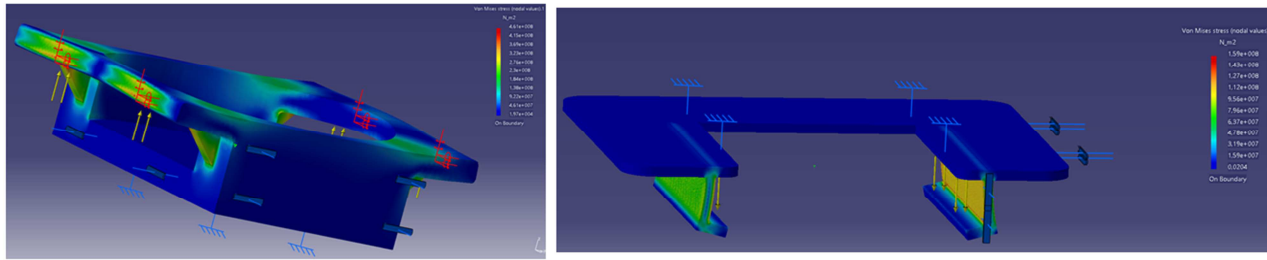
Figure 8. Simulation results.
