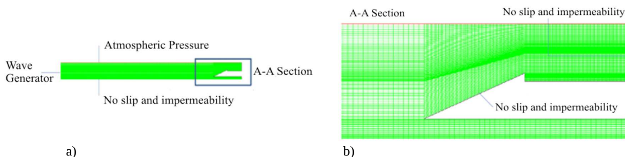
Figure 4. Spatial discretization applied to the onshore real scale overtopping device.
