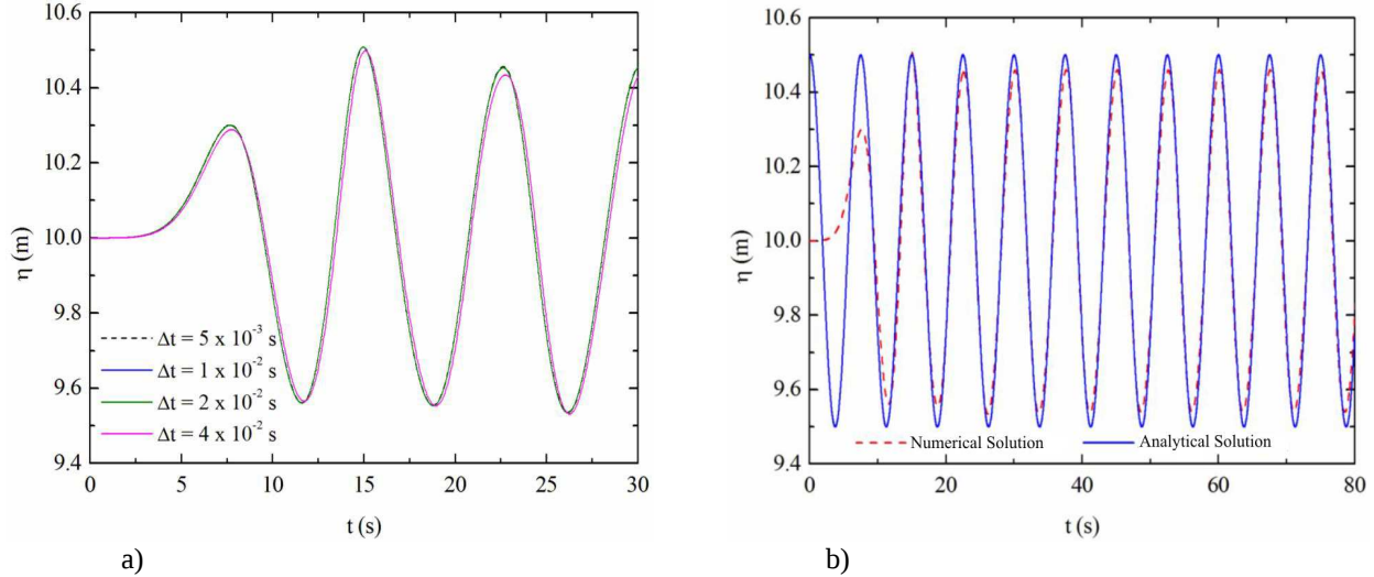
Figure 5. Numerical evaluation of the employed methodology: a) study of independent time step, b) verification of the numerical solution with the analytical solution presented in Chakrabarti (2005).
