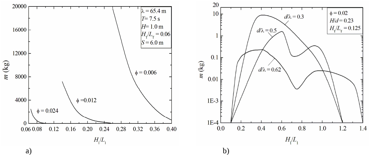
Figure 6. Effect of the ratio H_1/L_1 over the amount of mass entering into reservoir: a) present work for a real scale onshore device with different values of \phi ; b) onshore device in laboratory scale (Dos Santos et al., 2014).
