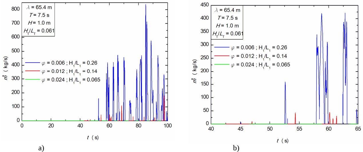
Figure 7. Instantaneous mass flow rate of water as function of time for three different values of \phi investigated: a) time interval of 0.0 \text{ s} \leq t \leq 100.0 \text{ s} , b) time interval of 40.0 \text{ s} \leq t \leq 65.0 \text{ s} .
