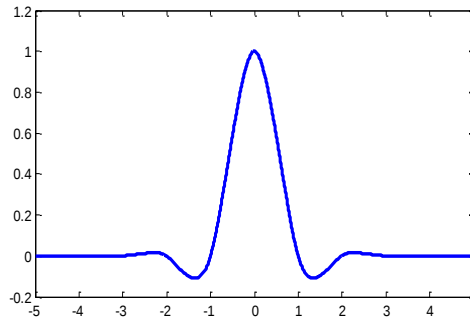
Figure 1. Interpolet IN4 scaling function.
