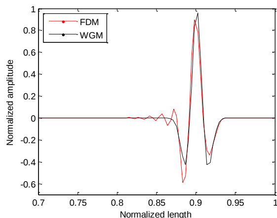
Figure 3. FDM and WGM results for \omega=80\text{Hz}
