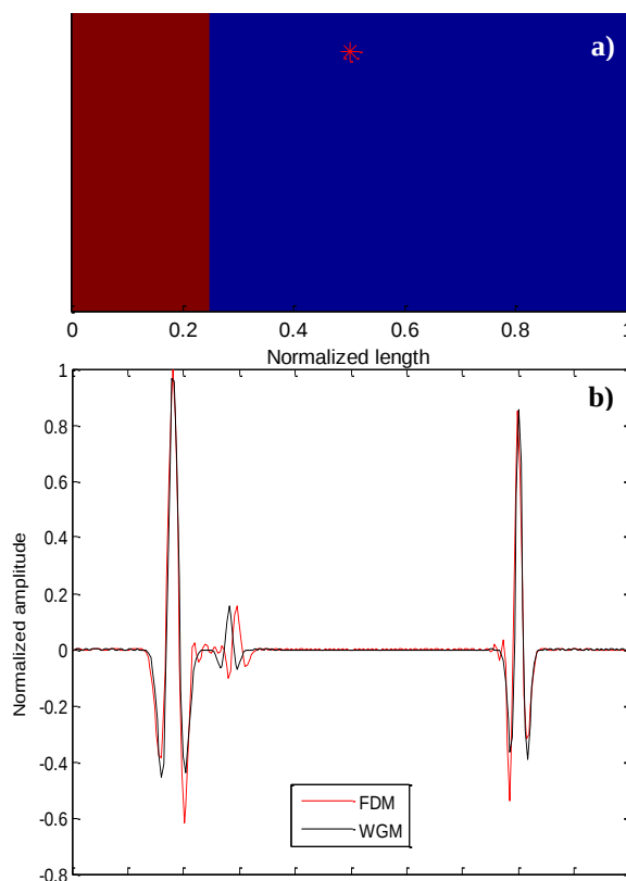
Figure 4. (a) Velocity profile (red region is a faster medium) and source position; (b) Snapshot for amplitude comparison at time t=0.35\text{ s}
