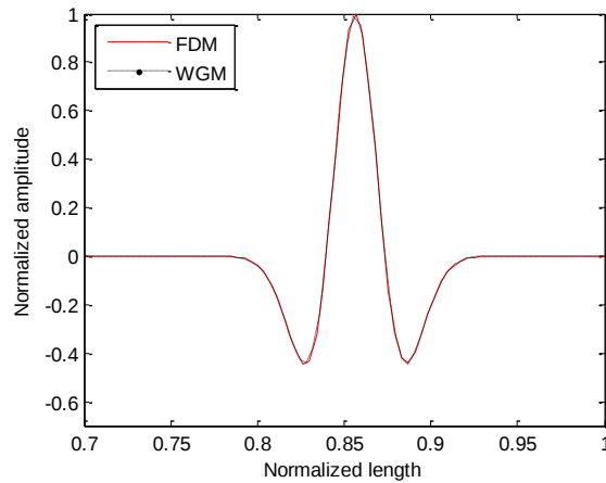
Figure 2. FDM and WGM results for \omega=40\text{Hz}
