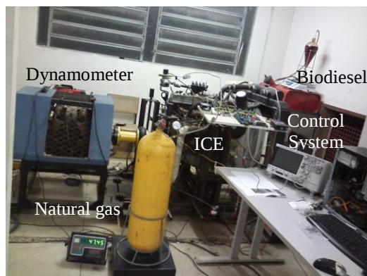
Figure 2. Engine MWM 4:07 TEC fed by natural gas or biodiesel, couplet to dynamometer electric LOGS
