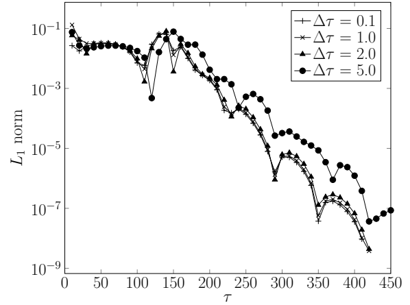
(b) Case 2: \Delta X = 1 , 128 \times 128 points in a domain 128 \times 128
