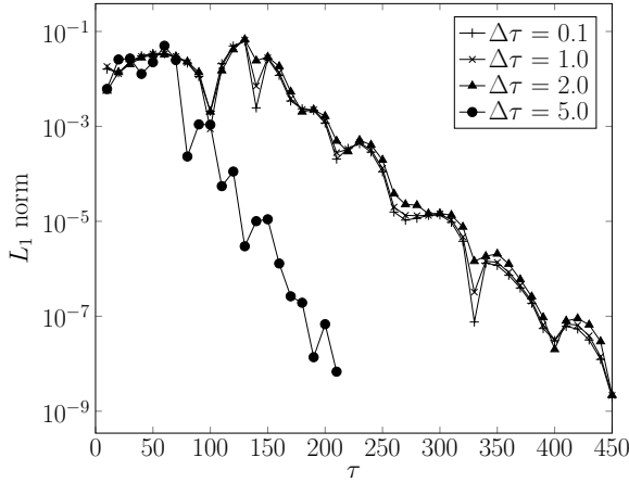
(a) Case 1: \Delta X = 2 , 64 \times 64 points in a domain 128 \times 128
