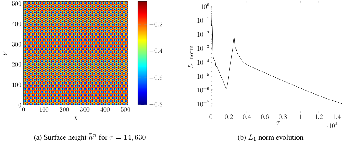
Figure 4: Numerical solution for a 2D anisotropic DKS equation - Stationary hexagonal structure, \alpha = 0.15
