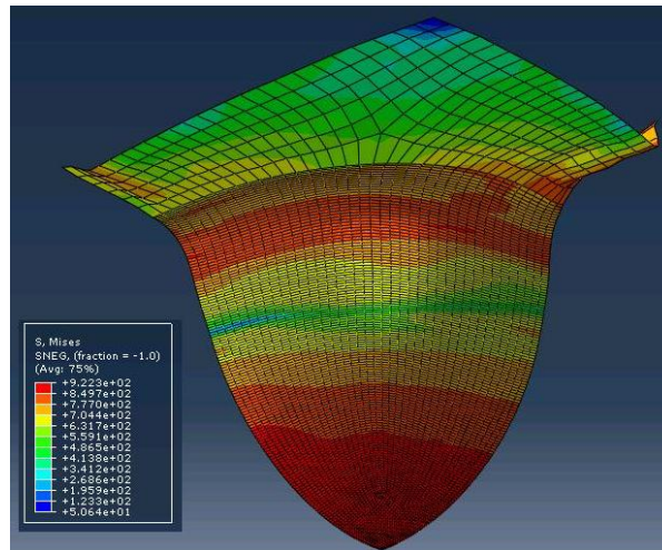
Figure 5. Simulation Results for speed 1.135 \text{ mm.s}^{-1}
