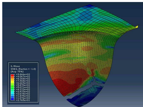
Figure 6. Simulation Results for speed 1.146 \text{ mm.s}^{-1}
