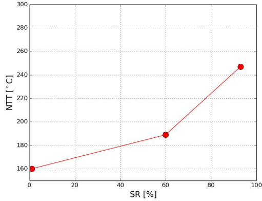
Figure 6 - NTT vs. Substitution Rate
