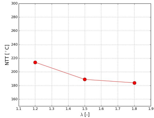
Figure 9 - NTT vs. relative air/fuel ratio
