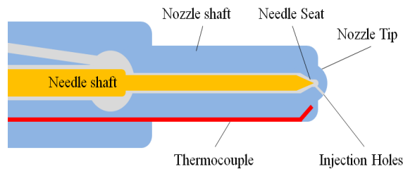
Figure 4 - Scheme of diesel injector nozzle instrumented with thermocouple reaching the tip area.
