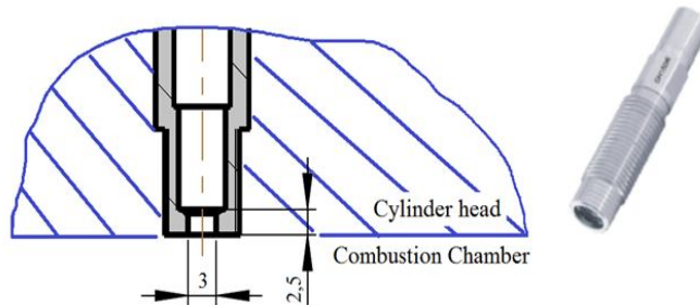
Figure 5 - Piezoelectric pressure sensor and installation details at engine cylinder head
