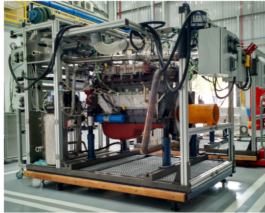
Figure 3 - Engine at Test Bench Trolley
