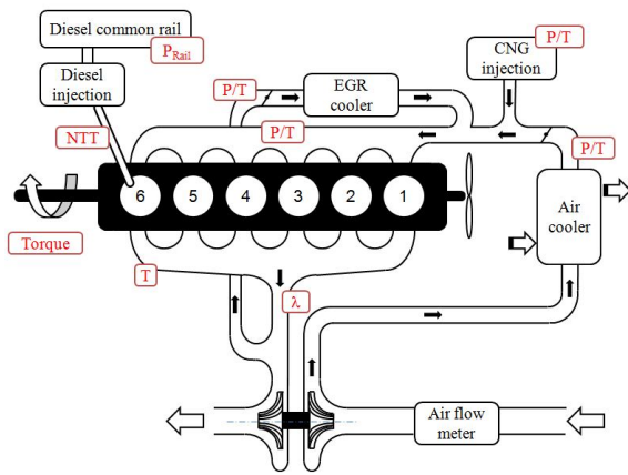
Figure 2 - Engine layout and main measurement points
