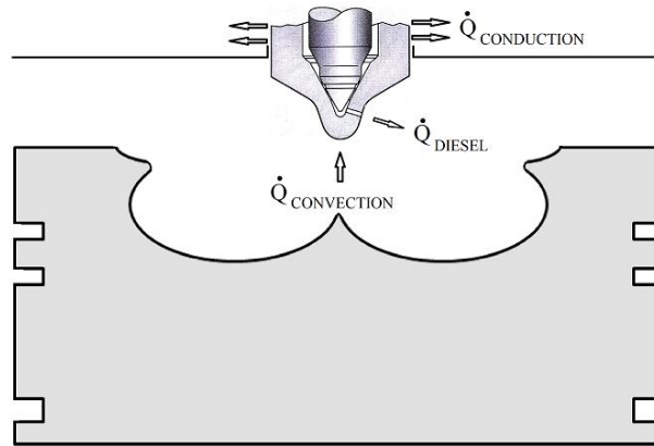
Figure 1 - Global heat transfer process at diesel nozzle
