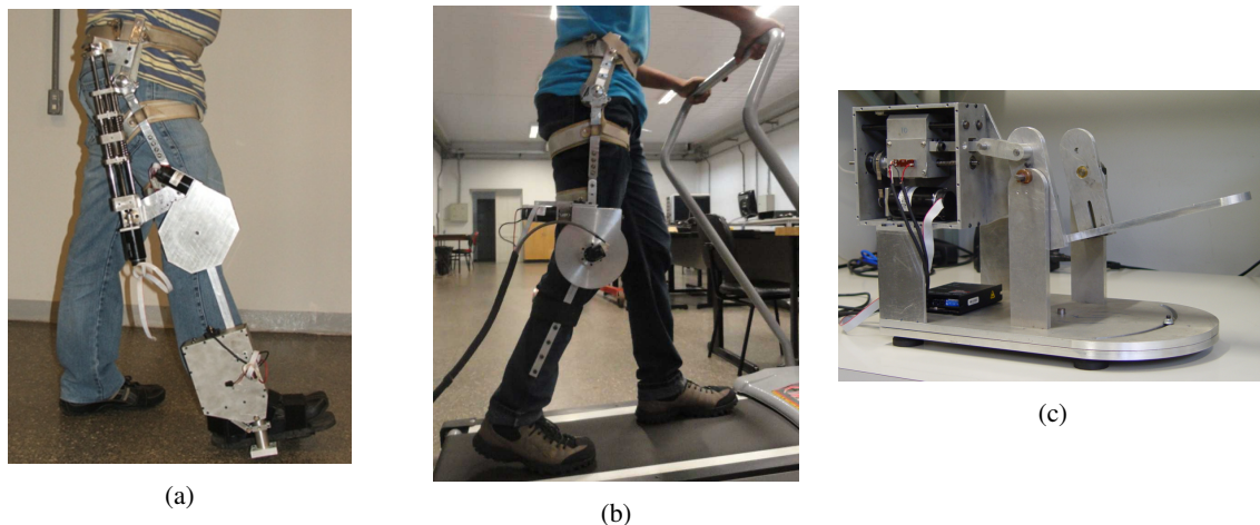
Figure 1: ReRob rehabilitation devices: (a) Exo-Kanguera (Jardim et al. , 2012); (b) knee orthosis (Santos and Siqueira, 2014); (c) RePAiR (Robotic Platform for Ankle Rehabilitation) (Gonçalves, 2013, 2014).
