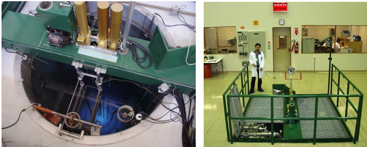
Figure 1. The IPR-R1 TRIGA reactor
