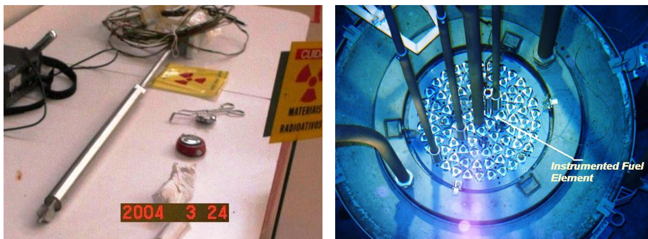
Figure 3. Instrumented fuel element before and after it was been positioned in the IPR-R1 reactor core.
