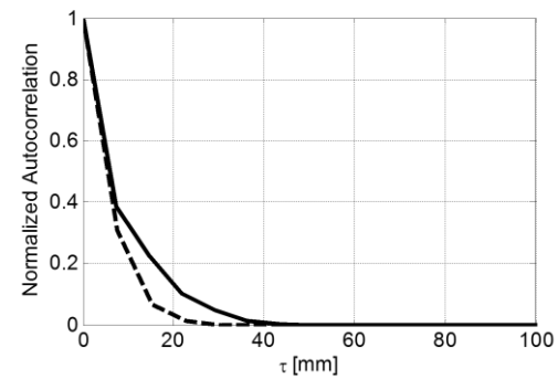
Figure 2. Normalised autocorrelation function in the x-axis R(\tau, 0)/R(0,0) (dashed line) and in the y-axis R(0, \tau)/R(0,0) (full line), for the (a) single and (b) double layer panel estimated from the area density spatial distribution.
