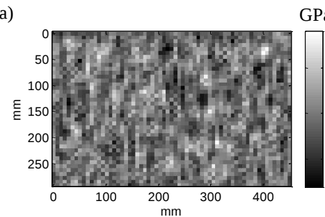
Figure 4. A numerically generated sample of the Young's modulus, in GPa, from the KL expansion and the estimated correlation function from the (a) single and (b) double layer panel.
