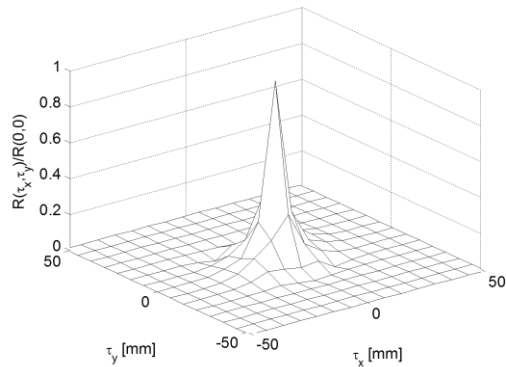
Figure 1. Normalized autocorrelation function R(\tau_x, \tau_y)/R(0,0) from the area density AW spatial distribution of the (a) single and (b) double layer panel.
