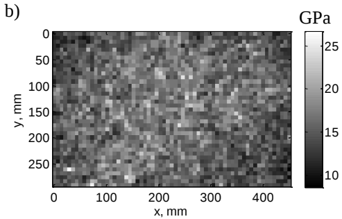
Figure 3. The Young's modulus in GPa from the optical measurements and the applied rule of mixtures at the (a) single and (b) double layer panel.
