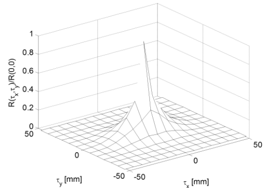
Figure 1. Normalized autocorrelation function R(\tau_x, \tau_y)/R(0,0) from the area density AW spatial distribution of the (a) single and (b) double layer panel.
