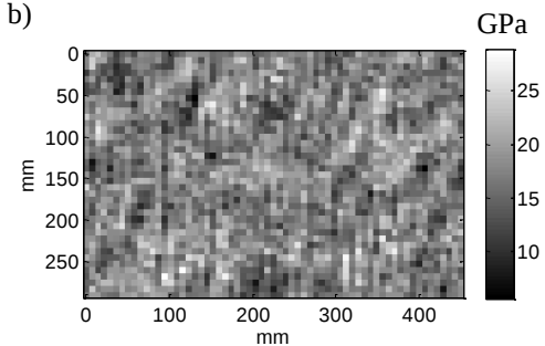
Figure 4. A numerically generated sample of the Young's modulus, in GPa, from the KL expansion and the estimated correlation function from the (a) single and (b) double layer panel.
