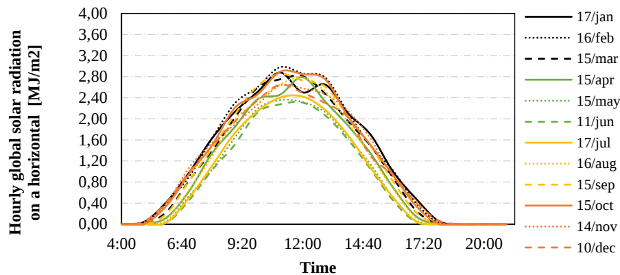
Figure 3. Monthly average hourly horizontal radiation
