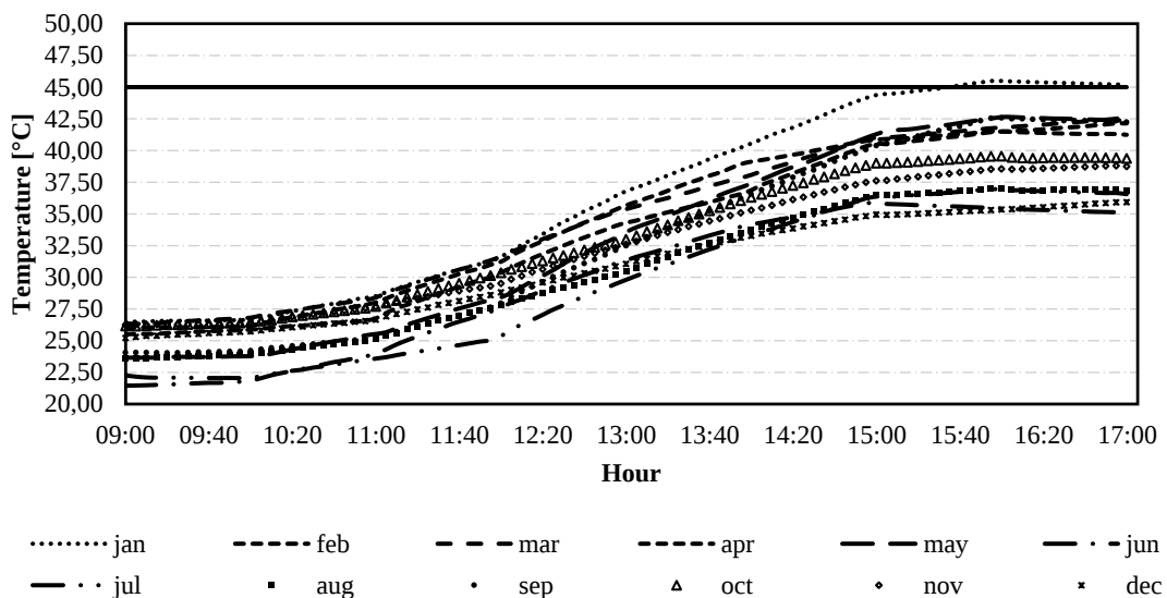
Figure 6. Temperature in the tank (200 l) during the simulation
