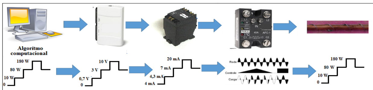
Figure 2. Illustration of the control for activating the simulating resistance
