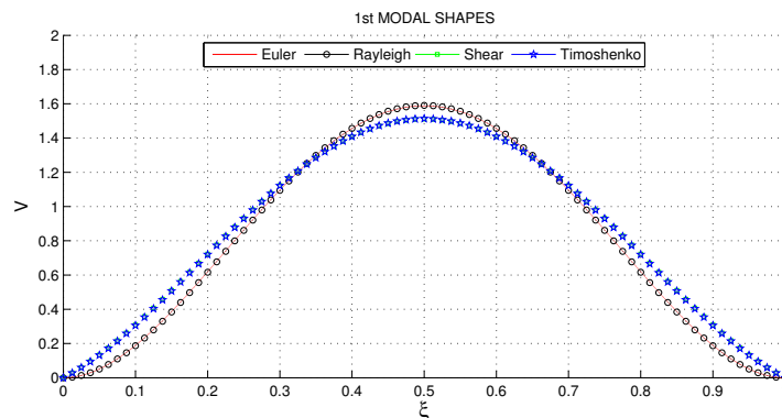
Figure 6. First modal shapes for clamped-clamped beam
