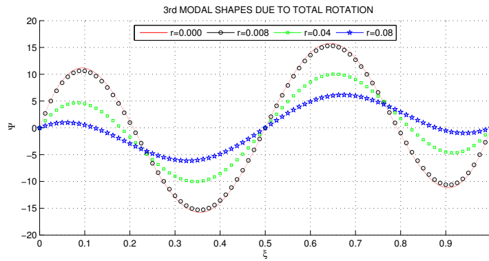
Figure 5. Third modal shapes due to complete rotation
