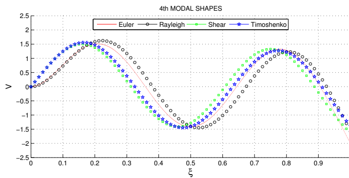
Figure 14. Fourth modal shapes for clamped-free beam
