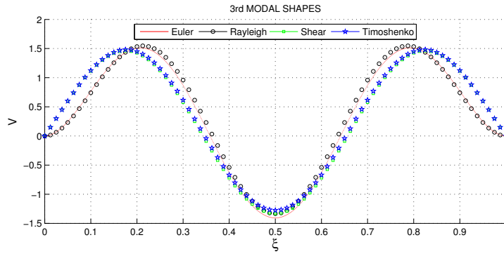
Figure 8. Third modal shapes for clamped-clamped beam
