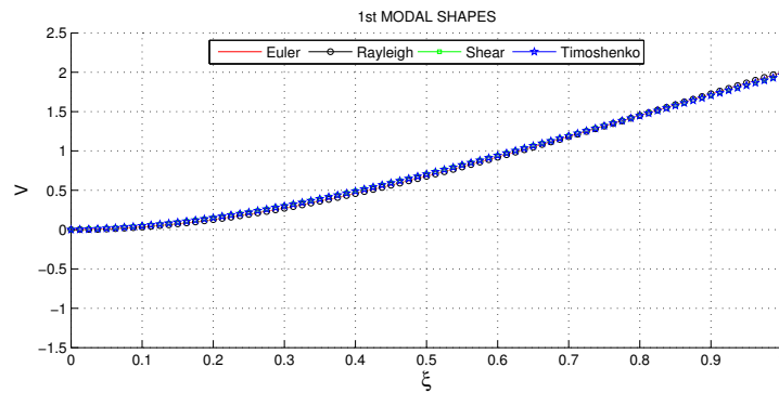
Figure 11. First modal shapes for clamped-free beam
