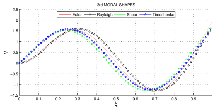
Figure 13. Third modal shapes for clamped-free beam
