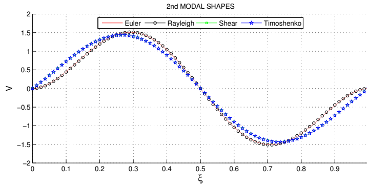
Figure 7. Second modal shapes for clamped-clamped beam
