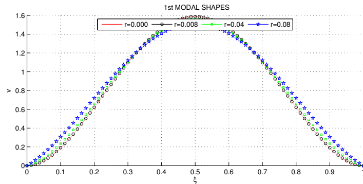
Figure 2. First modal shapes for clamped-clamped beam
