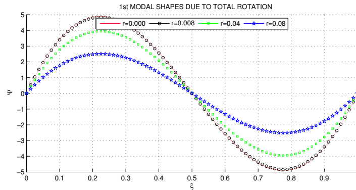
Figure 4. First modal shapes due to complete rotation
