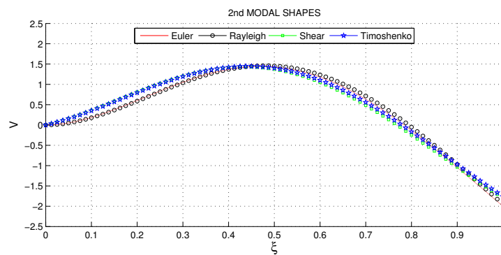
Figure 12. Second modal shapes for clamped-free beam
