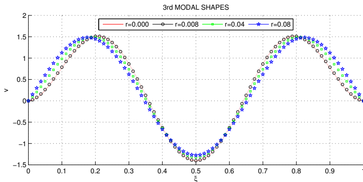
Figure 3. Third modal shapes for clamped-clamped beam
