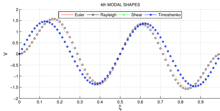
Figure 9. Fourth modal shapes for clamped-clamped beam
