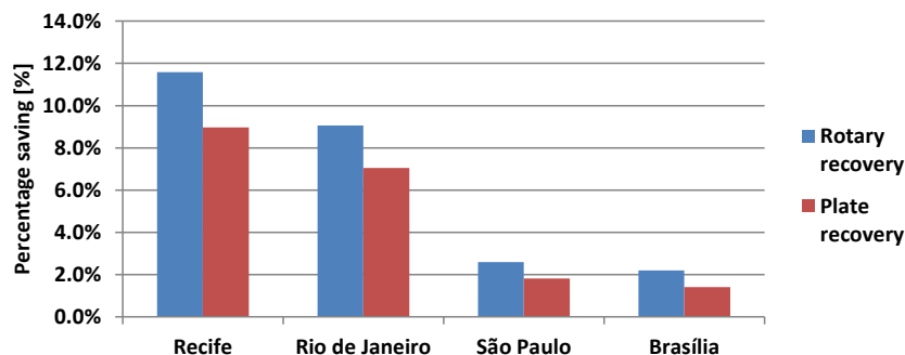
Figure 7. Percentual reduction of air conditioner system for each type of heat recovery and for each city.
