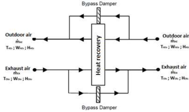
Figure 3. Schematic of the heat exchange
