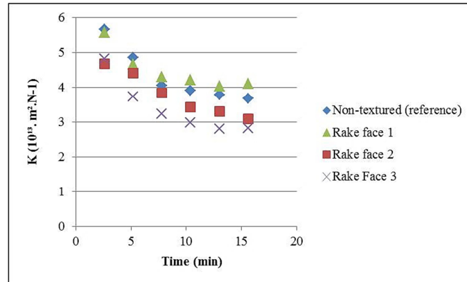
Figure 4. Wear coefficient (K) as function of the test time. N = 1.25 \text{ N} and n = 37.6 \text{ rpm} .
