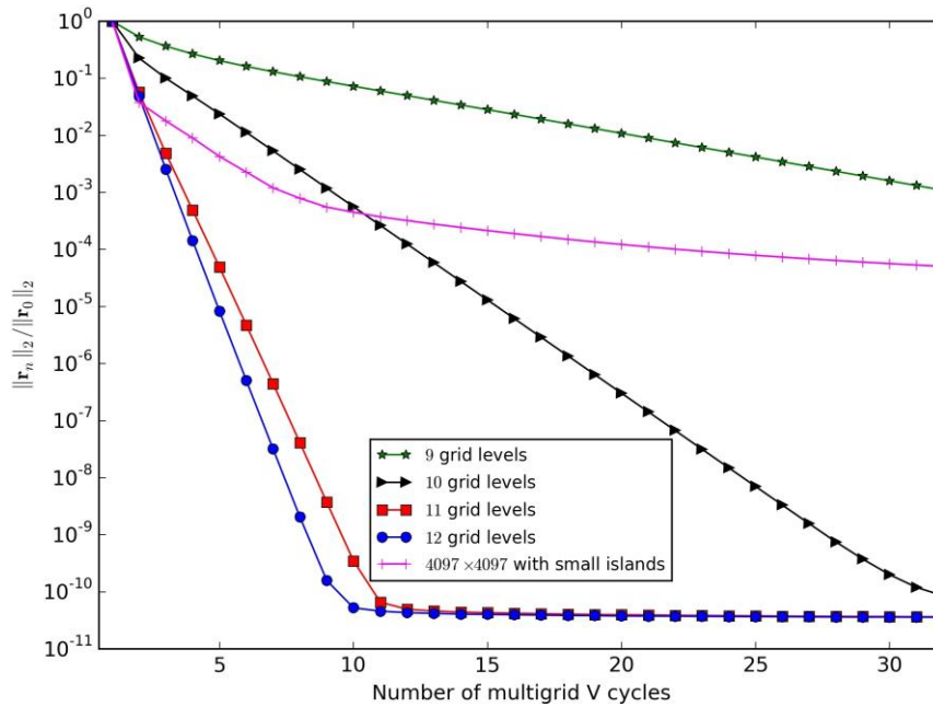
Figure 5. Decrease in the residual for different grid levels for the test case with N = 4097 \times 4097
