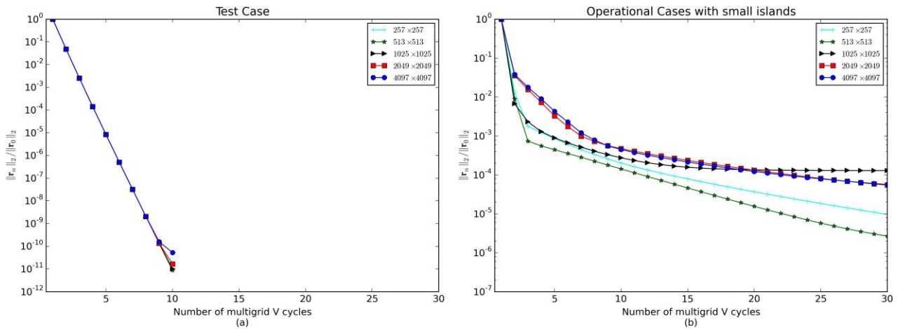
Figure 4. Decrease in the residual for test case (a) and operational cases (b) with "small islands"
