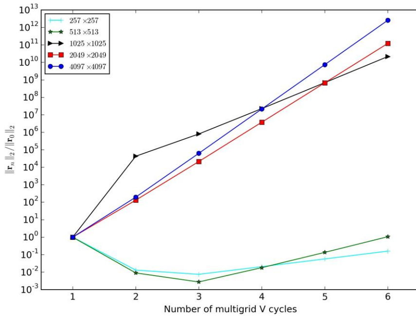
Figure 3. Increase in the residual for cases with "small islands"
