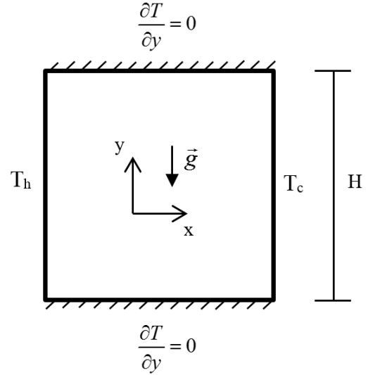
Figure 2: General schematic configuration
