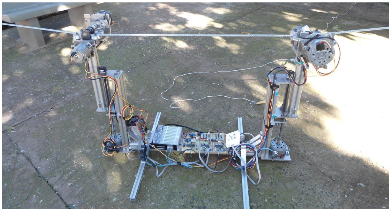
Figure 10. Robot in cable locomotion test
