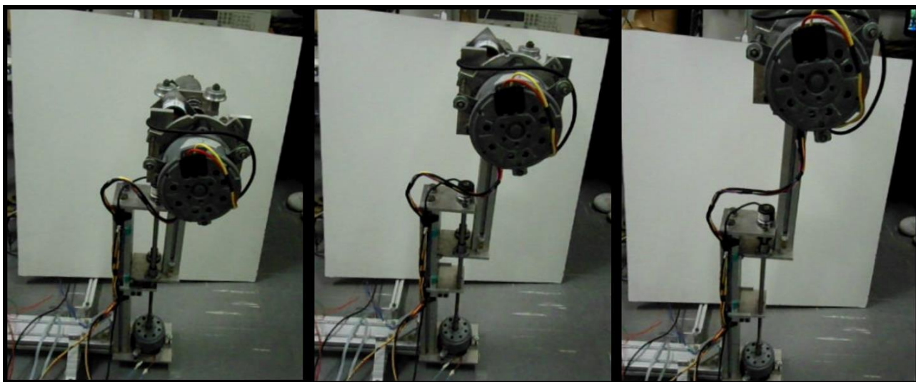
Figure 9. Robot leg contraction/expansion test
