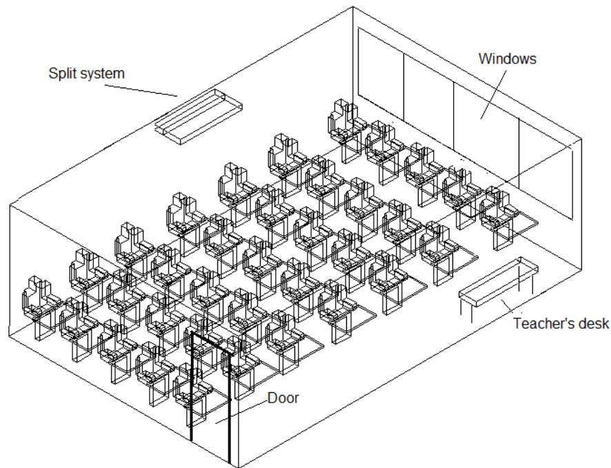
Figure 1. Classroom geometry
