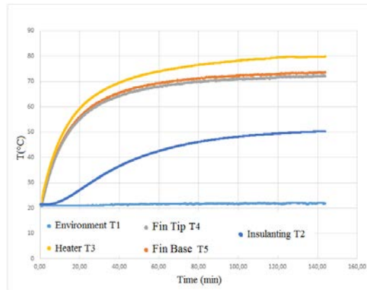
Figure 5. Temperature variation in time for the five thermocouples of Fig. 1.
