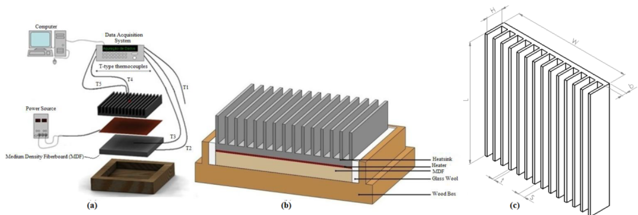
Figure 1. (a) Arrangement of test bench, (b) details of the heatsink and (c) heatsink geometric parameters.
