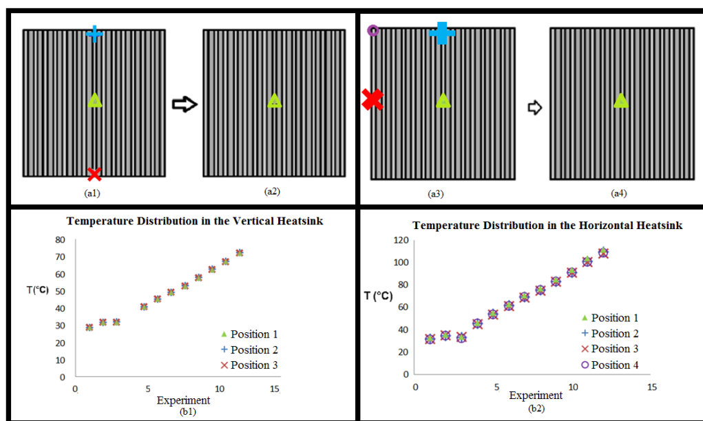
Figure 3. (a1) and (a3) positions of the thermocouples during the distribution test; (a2) and (a4) positions of the thermocouples in the other tests; and (b1) and (b2) refer to temperature distribution of each thermocouple.
