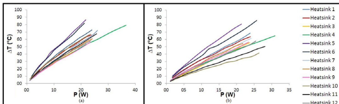
Figure 7. Temperature variation in relation to the power supply a) for horizontal and b) for vertical heat sinks.
