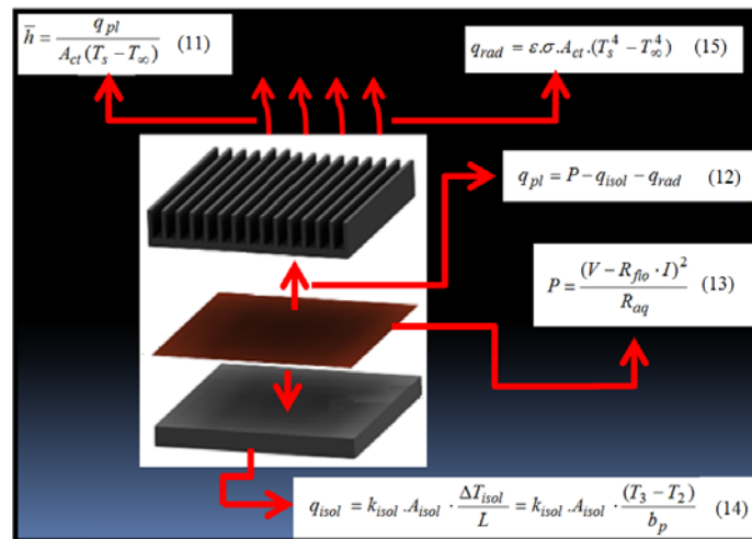
Figure 4. Heat distribution illustration in the experimental set.
