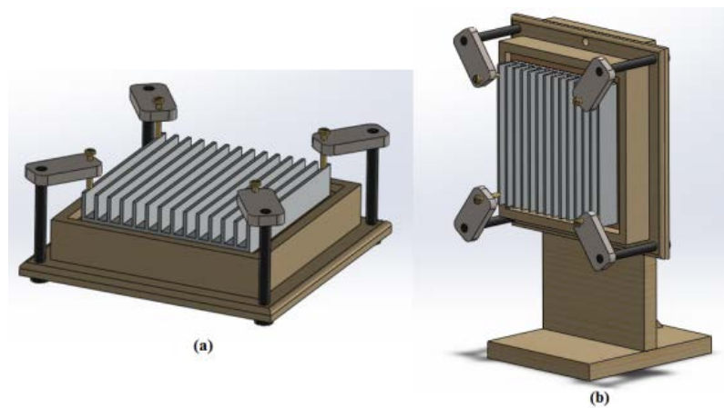
Figure 2. (a) Horizontal and (b) vertical heat sink assemblies.
