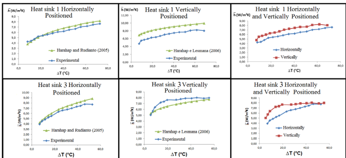
Figure 6. Heat transfer coefficient variation in temperature for Heat sinks 1 and 3.
