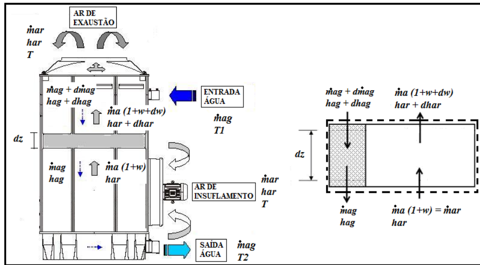
Figure 8. Filling volume control in countercurrent.
