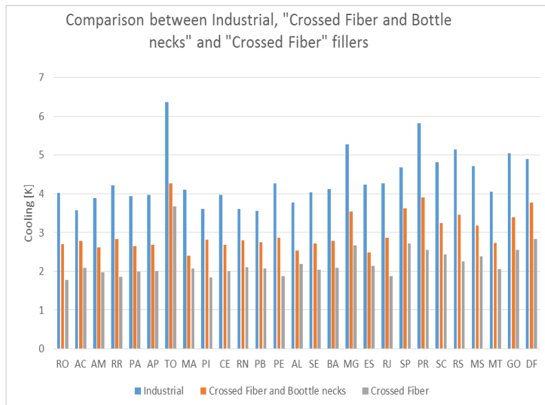
Figure 11. Comparison of Cooling (Figures 1 to 7).
