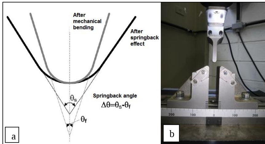
Figure 1. (a): Definition of springback angle (Lee et al, 2009). (b): Device mounted universal testing machine for testing three-point bending in air or Air bending test.
