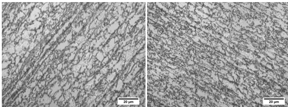
Figure 5. Optical microscopy after air bending test to 30 degrees for the DP 600. Reagent: Nital 2%. 500X.
