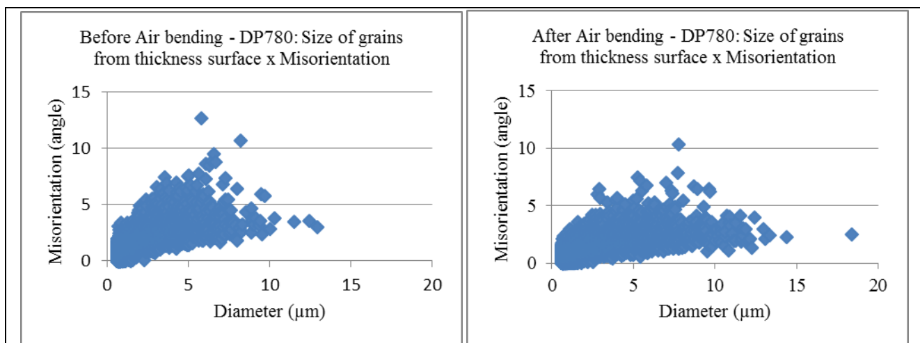
Figure 8. Dispersion relating the size of the grains with the misorientation angle for the steel DP 780, before and after sheet metal forming.
