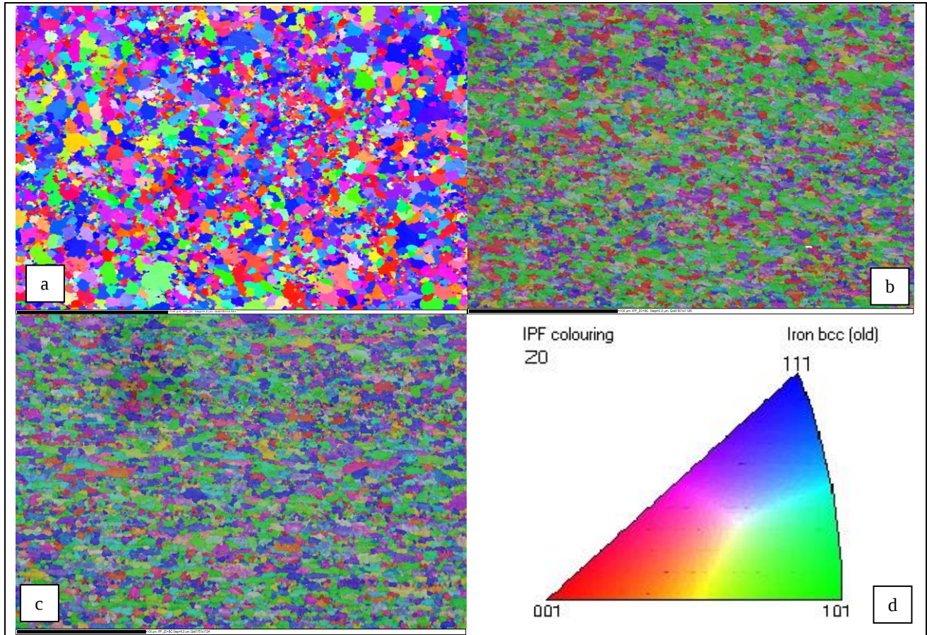
Figure 9. Crystallographic orientation plans for the DP 780. (a): Upper surface before air bending. (b): Thickness surface before air bending. (c): Thickness surface after air bending up to 30 degrees. (d): Legend indicating the Miller indices: crystallographic orientations.
