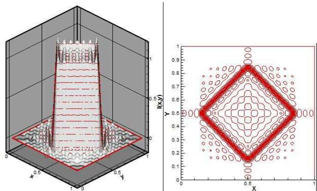
Figure 3. Distribution of Indicator Function in the domain of calculation, 3-D and 2-D views, for n = 20 .
