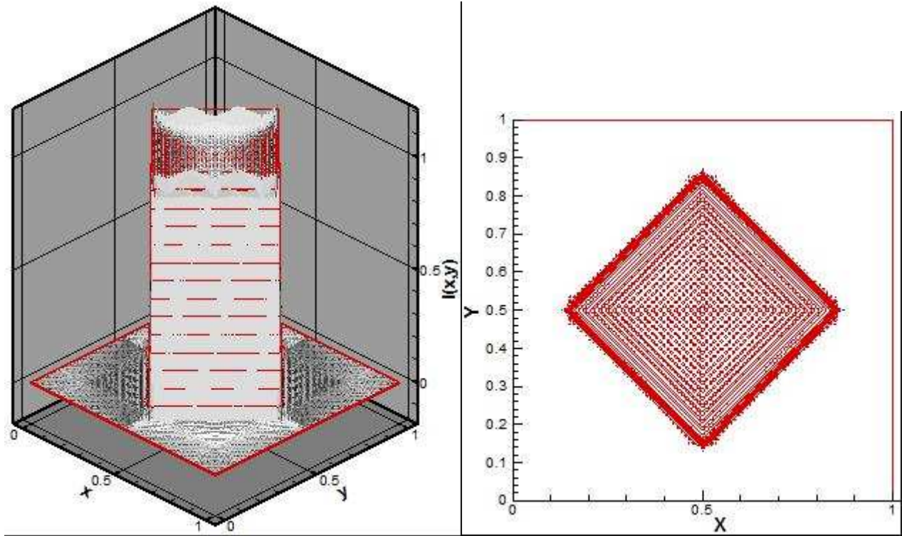
Figure 4. Distribution of Indicator Function in the domain of calculation, 3-D and 2-D views, for n = 100 .
