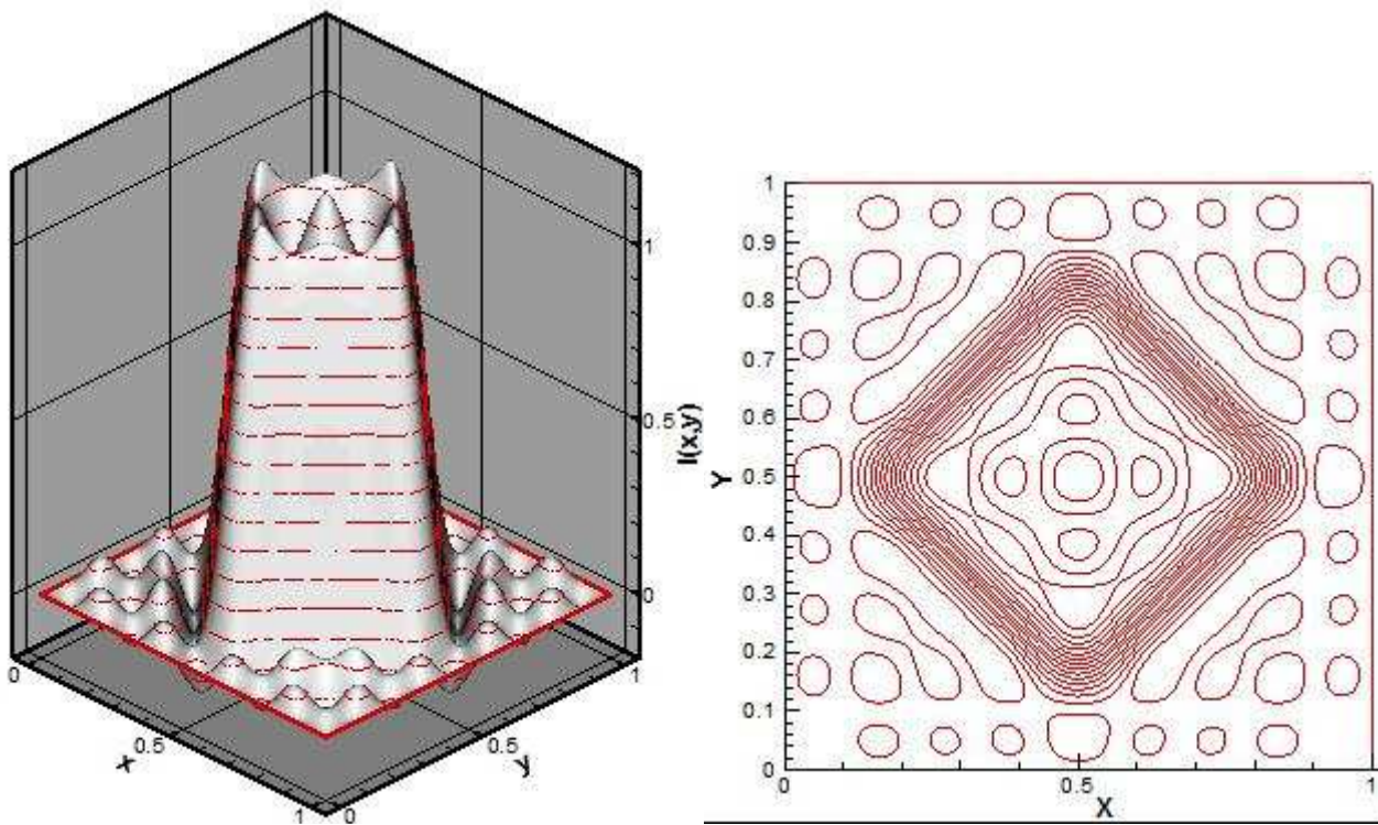
Figure 2. Distribution of Indicator Function in the domain of calculation, 3-D and 2-D views, for n = 10 .
