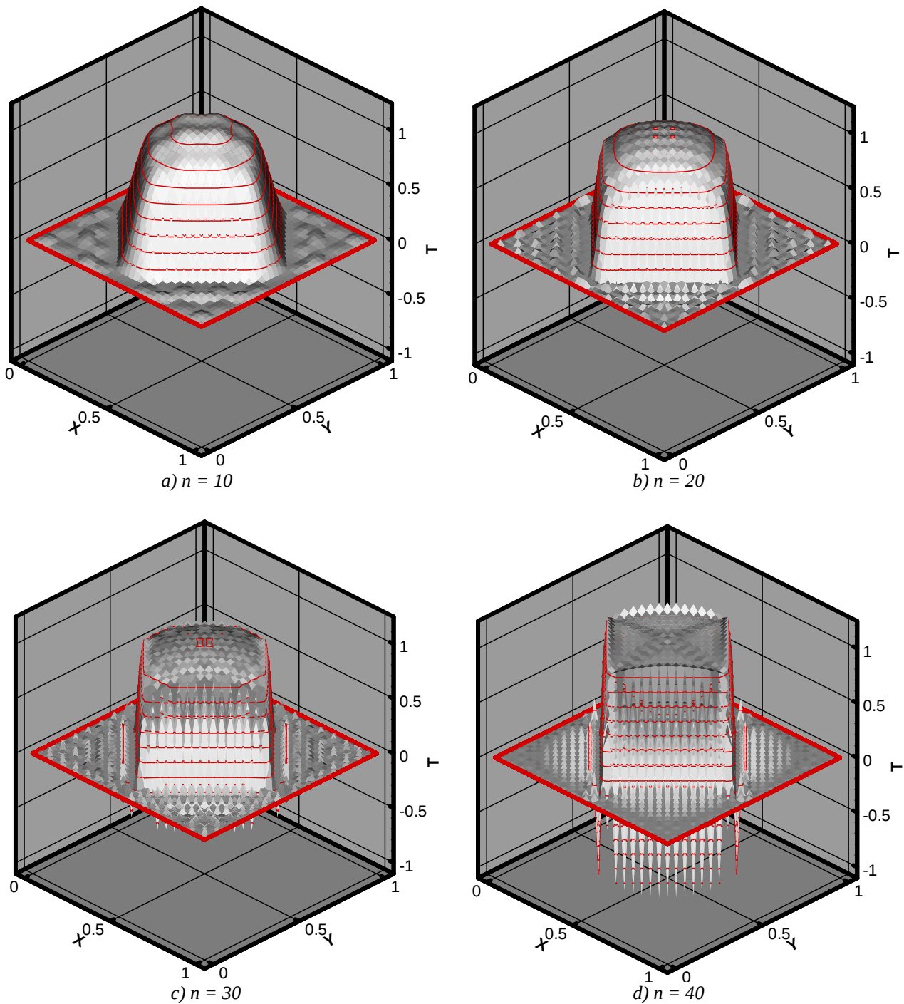
Figure 6. Temperature distribution for t = 0.01 .
