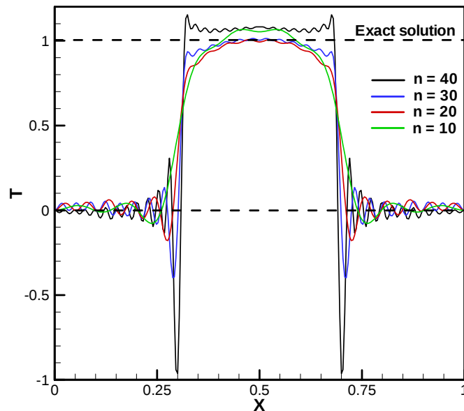
Figure 7. Convergence of temperature, for t = 0.01 .
