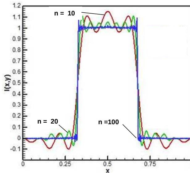
Figure 5. Convergence of Indicator Function, for y = 0.5 .
