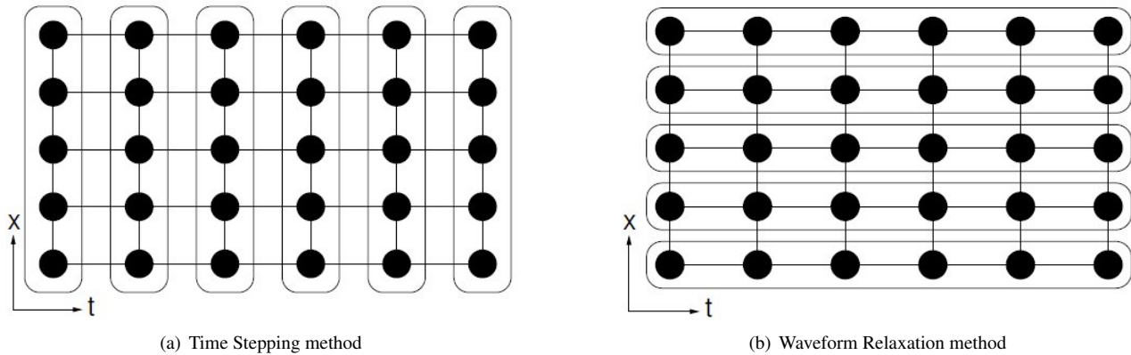
Figure 1. Update procedure of the unknowns in Time Stepping e Waveform Relaxation methods (Van Lent, 2006).
