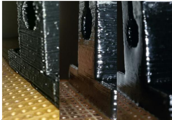
Figure 11 – Progress of smoothing along the object
