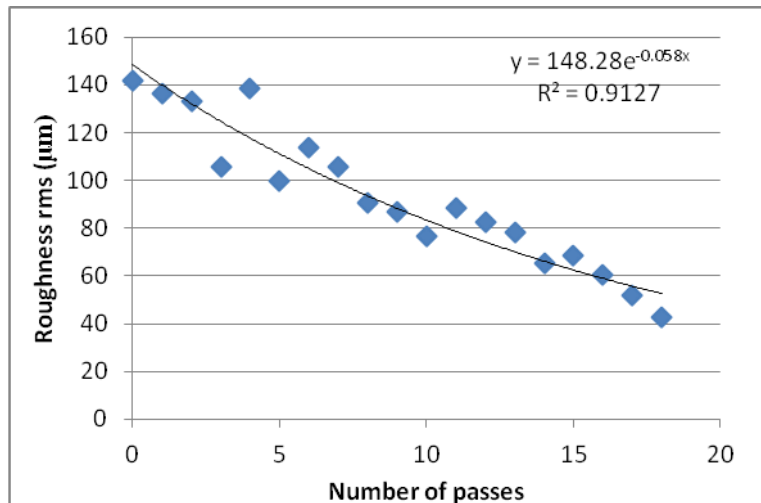
Figure 9 – Surface Roughness as a function of number of passes
