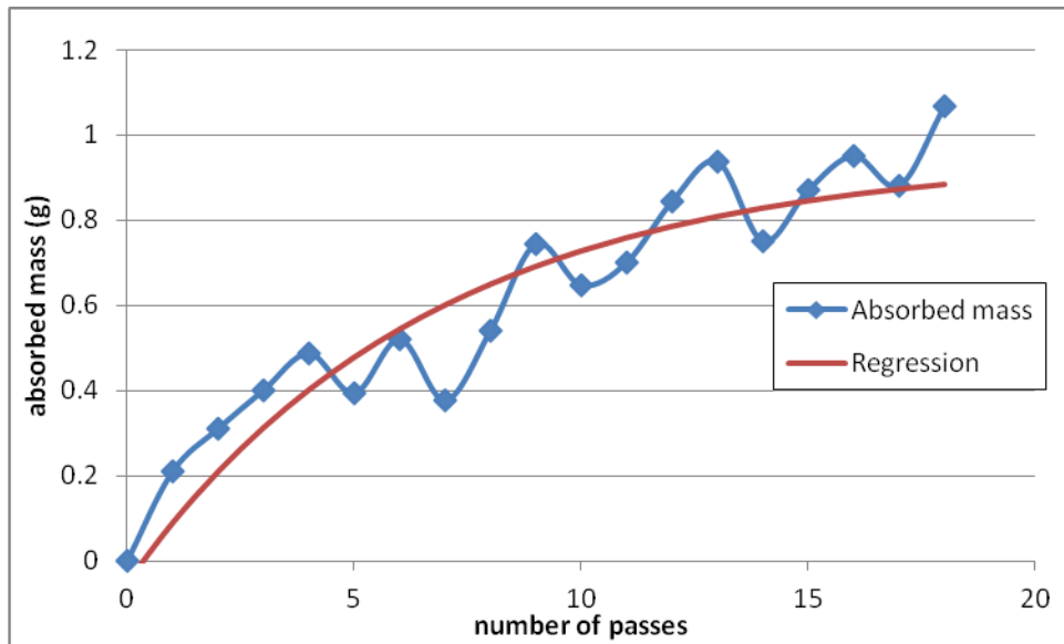
Figure 7 – Gravimetric analysis
