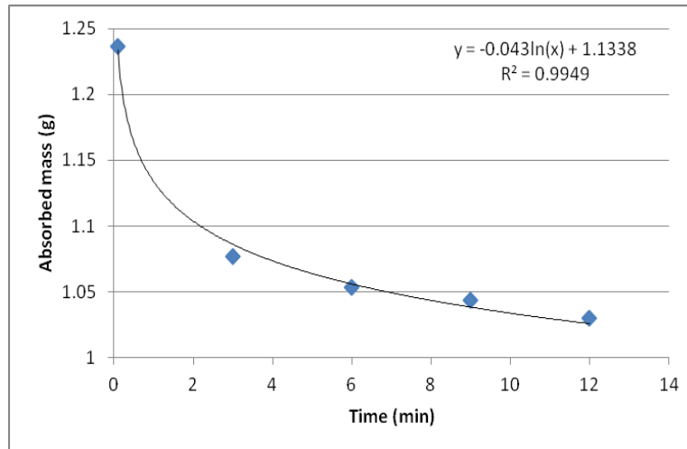
Figure 8 – Drying Gravimetric analysis of 13rd pass
