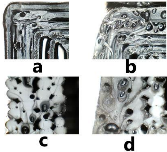
Figure 13 – Analysis of solvent attack depth in longitudinal and transversal specimen sections, where a) longitudinal section before attack; b) longitudinal section after attack (18 passes); c) transversal section before attack; d)transversal section after attack (18 passes)
