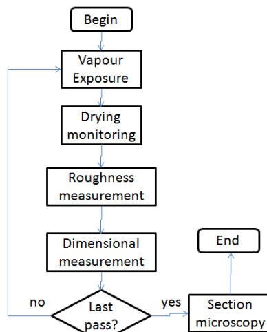
Figure 6 – Experiment flow chart
