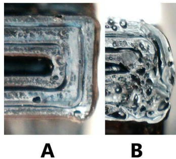
Figure 12 – Comparison between straight surface before and after vapour attack
