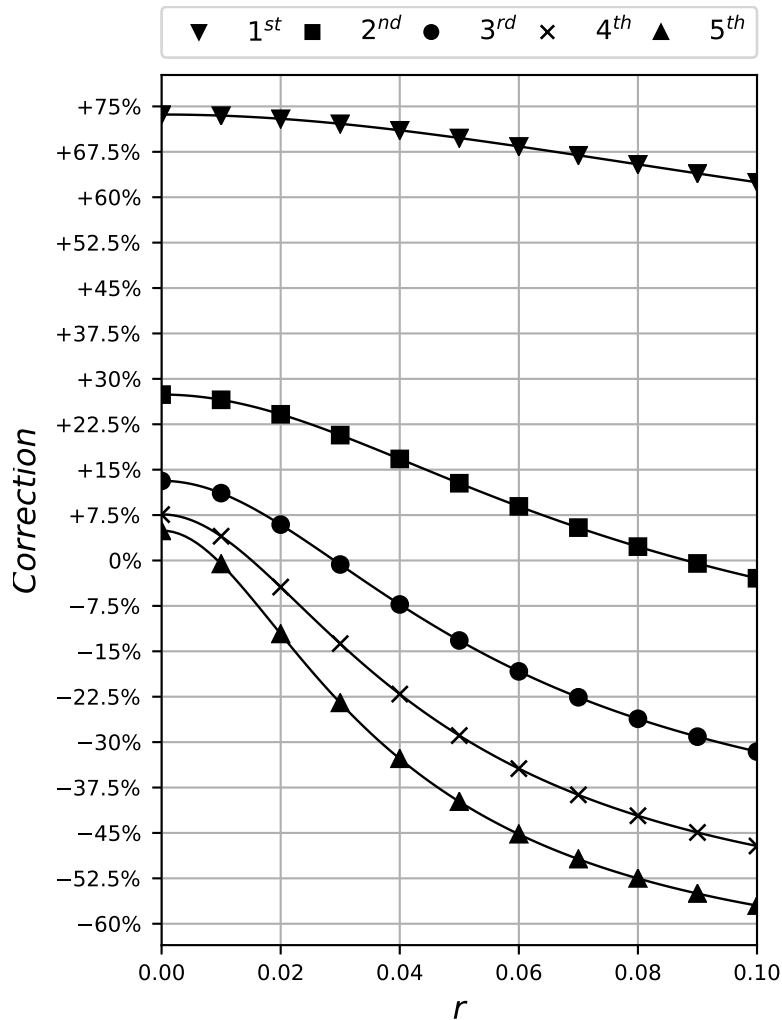
Figure 8: Correction in the natural frequencies of Euler-Bernoulli beam on Winkler foundation in comparison to Timoshenko beam on Pasternak foundation for some values of parameter r (FEM - 70e).
