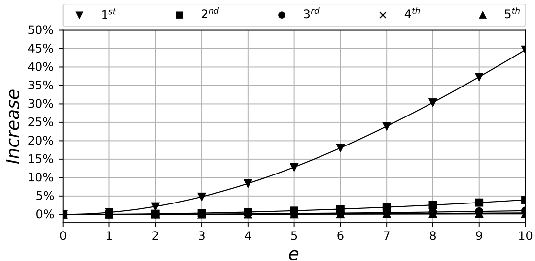
Figure 4: Increase in the natural frequencies of a beam on a Winkler ( p = 0 ) foundation for various values of parameter e (FEM - 70e).
