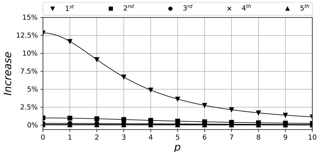
Figure 7: Influence of the foundation stiffness on a Pasternak foundation (FEM - 70e).
