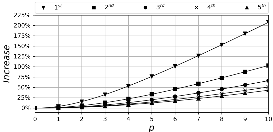
Figure 5: Increase in the natural frequencies of a beam on Pasternak ( e = 5 ) foundation considering the parameter p (FEM - 70e).
