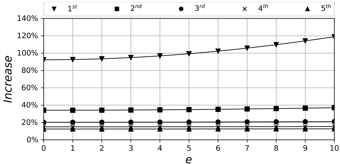
Figure 6: Increase in the natural frequencies of a beam on a Pasternak ( p = 5 ) foundation for various values of e (FEM - 70e).
