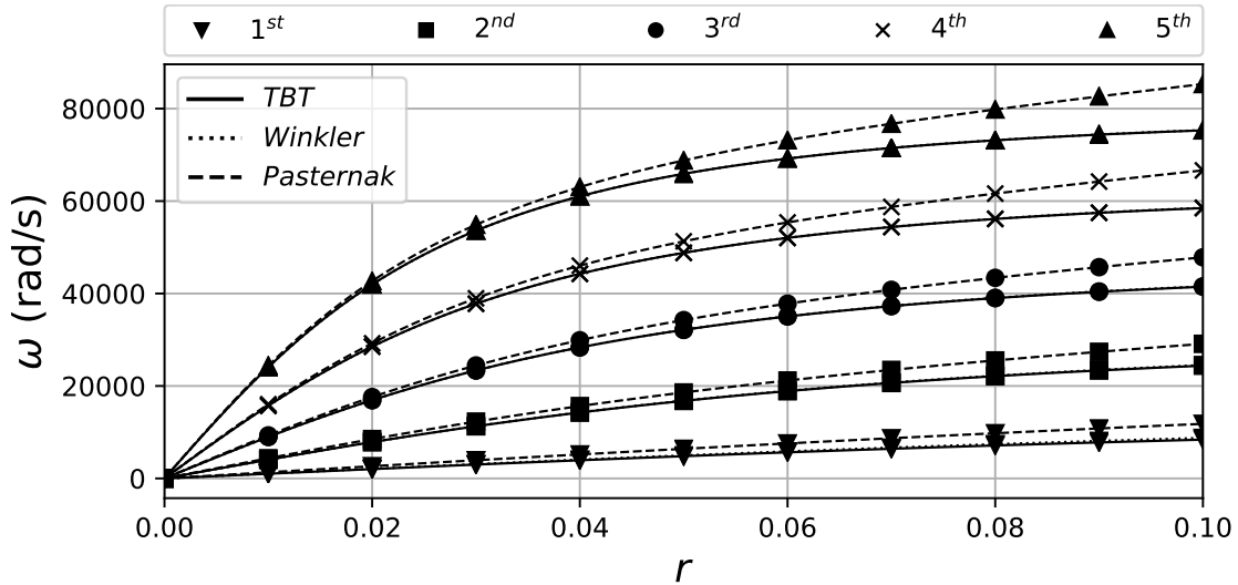
Figure 3: Frequency curves of beams on different elastic foundations (FEM - 70e).
