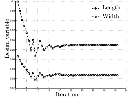
(b) Optimization progress of the design variable.
