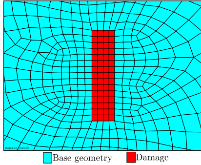
(c) Repaired geometry.
