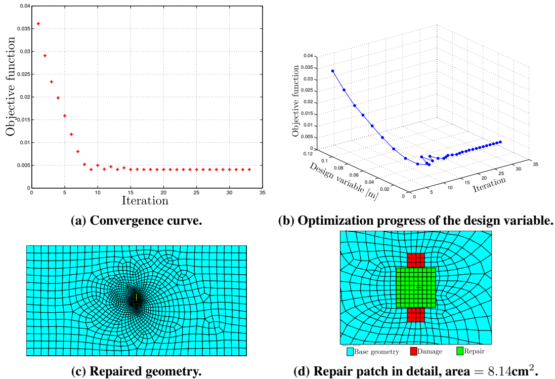
Figure 4: Optimum configuration with square repair with side l_r = 28.53\text{mm} .
