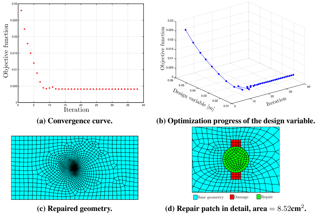
Figure 3: Optimum configuration with circular repair R = 16.47\text{mm} .
