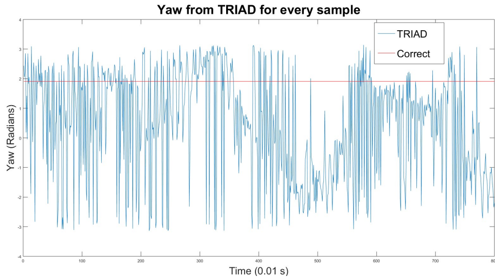
Figure 4. Yaw angles from TRIAD method for every data sample
