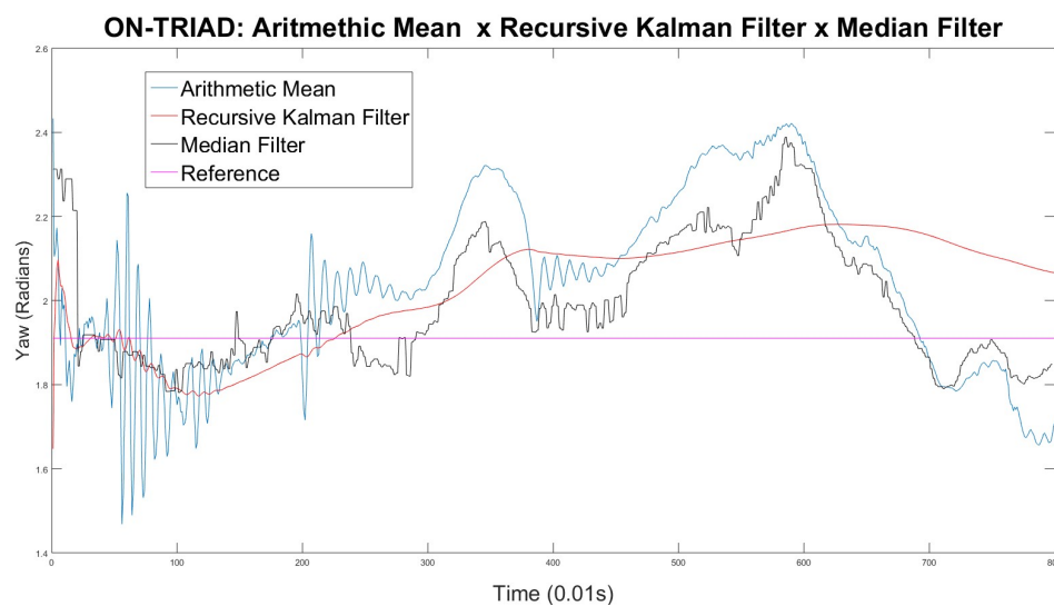
Figure 10. Comparison between the data handling influence in yaw angle result obtained with ON-TRIAD
