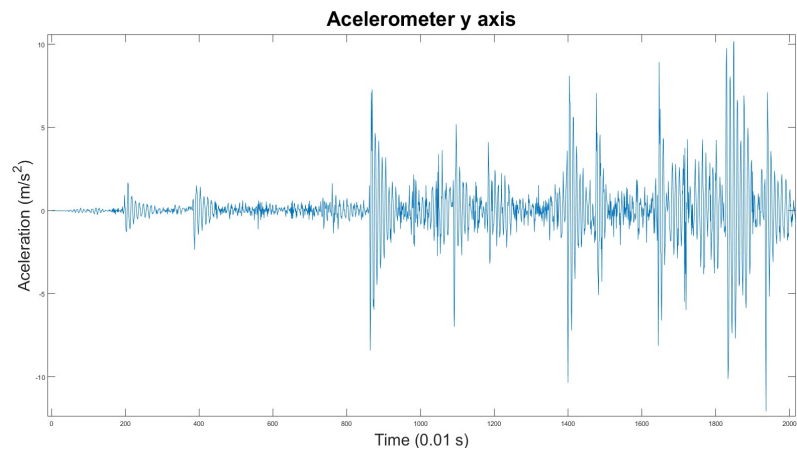
Figure 2. y axis accelerometer data
