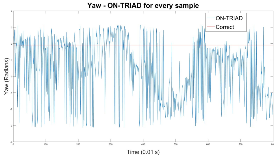
Figure 5. Yaw angles from ON-TRIAD method for every data sample
