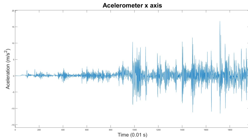
Figure 1. x axis accelerometer data
