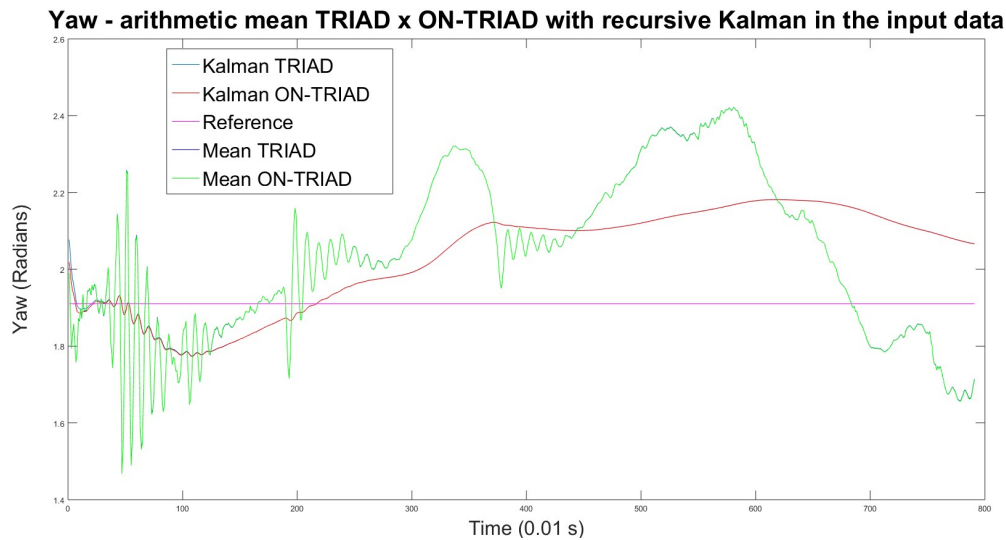
Figure 8. Yaw angles from TRIAD and ON-Triad methods with recursive Kalman filter in the input data
