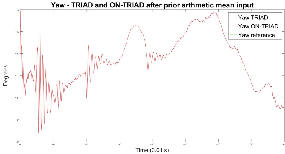
Figure 6. Yaw angles from TRIAD and ON-TRIAD methods for data with prior arithmetic mean
