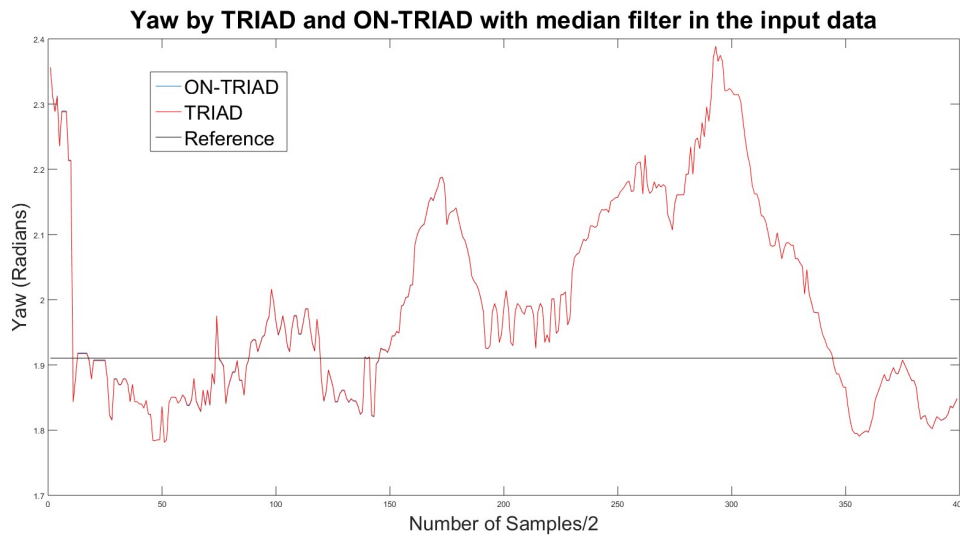
Figure 9. Yaw angles from TRIAD and ON-TRIAD methods with median filter in the input data
