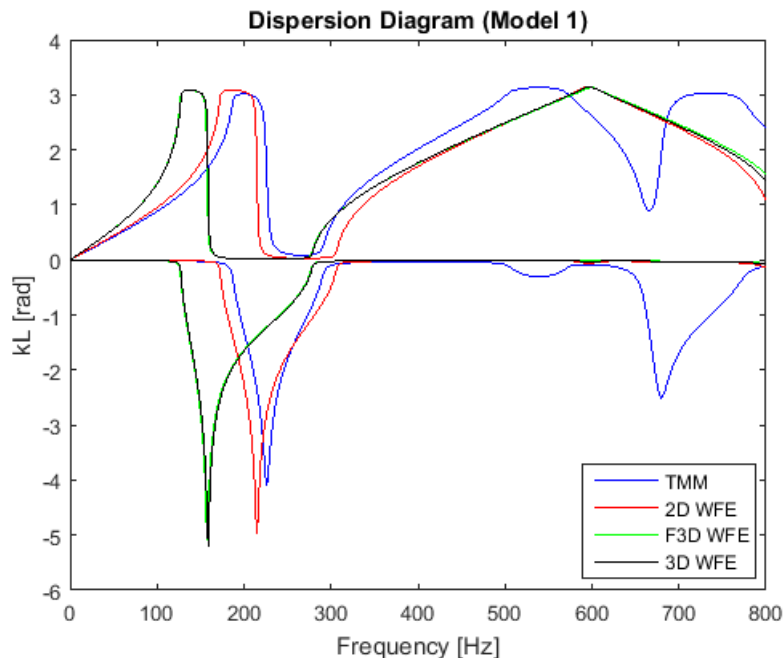
Figure 5. Dispersion diagram for Model 1 calculated by TMM and WFE with geometry: 2D, F3D and 3D.
