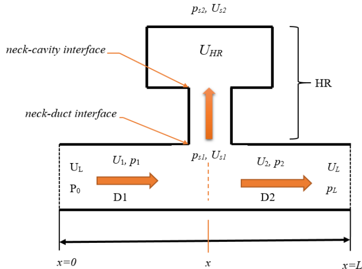
Figure 2. Sketch of the unit-cell duct-HR system.
