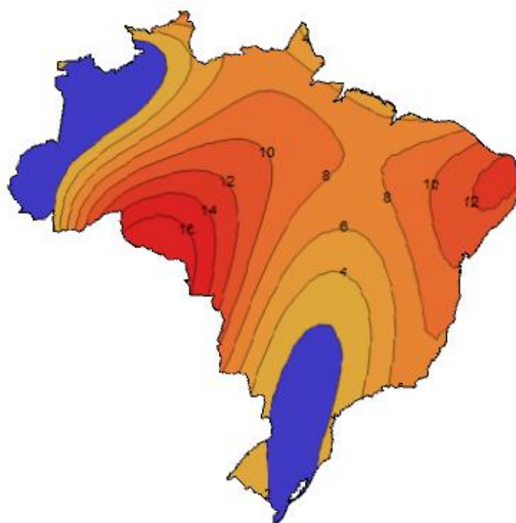
Figure 3. Probabilities of wind speeds proposed in ABNT NBR 6123:1988 being exceeded in a single year.
