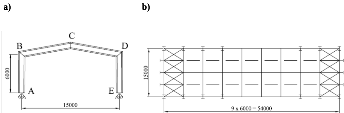
Figure 6. a) Front view of the steel frame, and b) top view of the industrial building.
