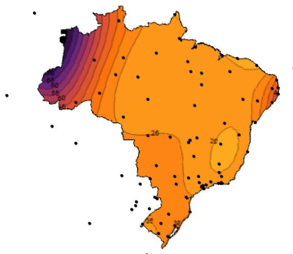
Figure 5. Simplified trend analysis charts of maximum annual winds speeds for extrapolation of 10 (a); 50 (b) and 100 (c) years, from 2016.
