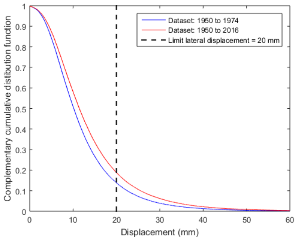
Figure 9. Horizontal displacement ( y ) complementary CDF ( P[Y \geq y] ) for SBSP Airport Station.
