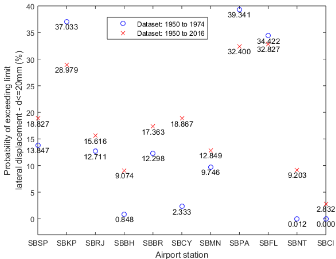
Figure 10. Failure probabilities for service limit state (lateral displacements) for different datasets and selected weather stations.
