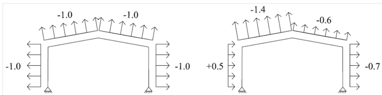
Figure 7. Combination of internal and external pressures coefficients.
