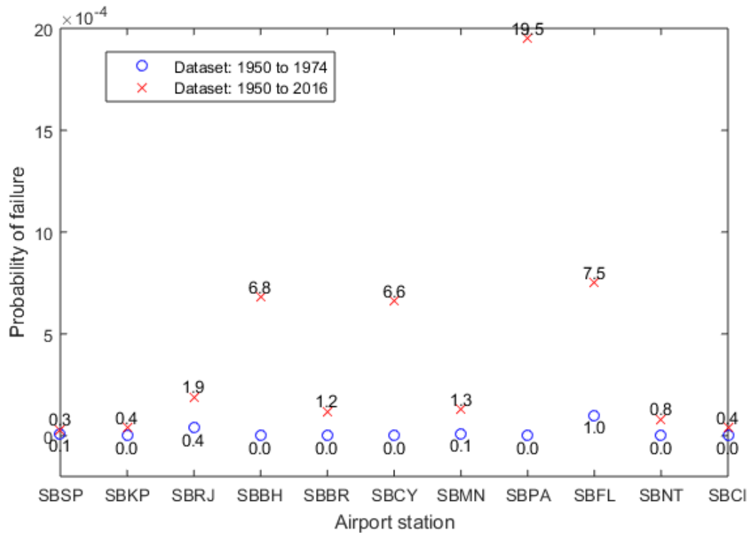
Figure 8. Failure probabilities for steel frames at different geographical locations (corresponding to weather stations as shown).
