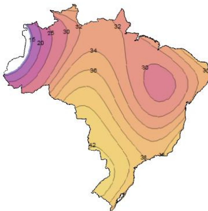
Figure 2. Updated basic wind speed chart for the Brazilian territory, dataset from 1950 to 2016.
