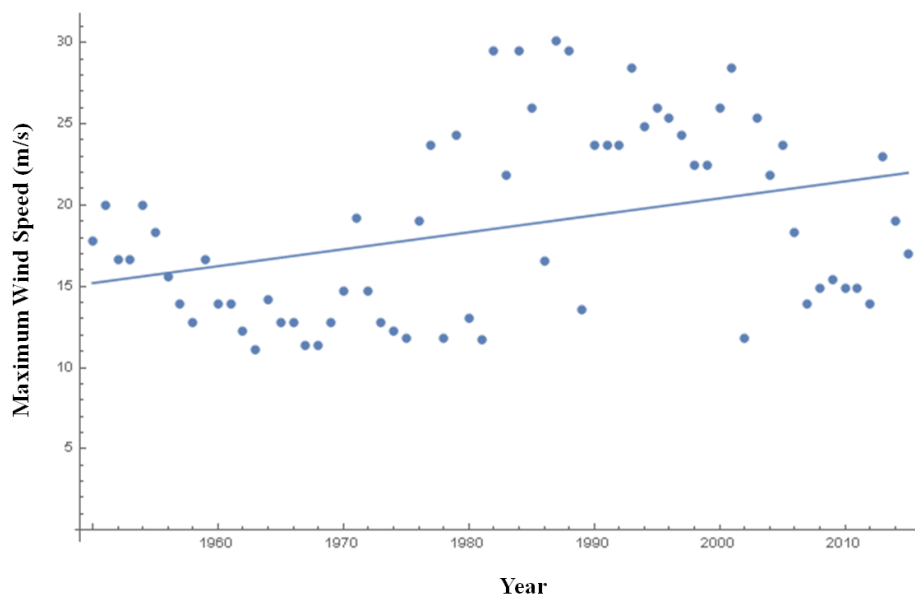
Figure 4. Example of linear fit showing mean trend of maximum annual wind speeds for SBMO station (Maceió).
