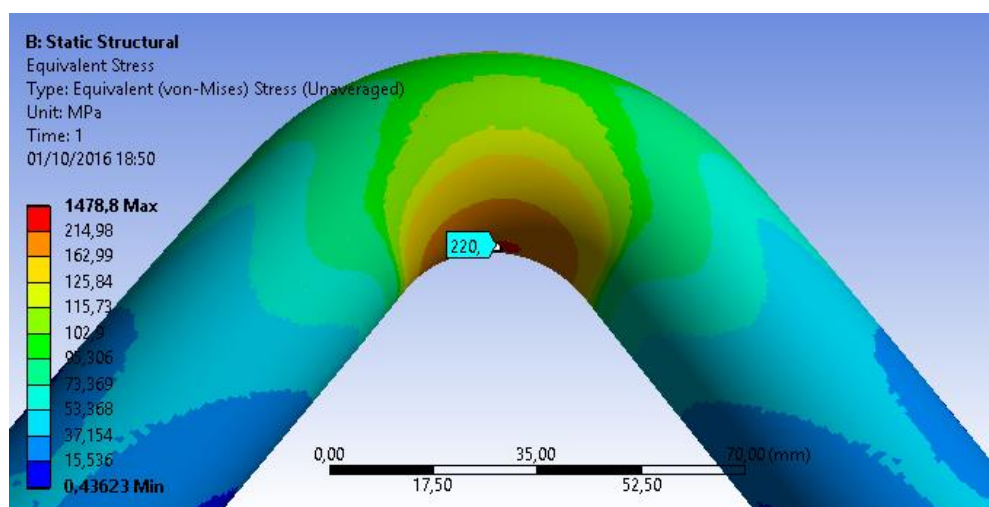
Figure 3 – Equivalent Stress von-Mises
