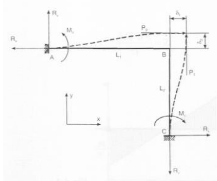
Figure 1 – Configuration of mathematical model
