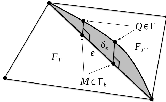
Figure 5: Construction of nodes Q \in \Gamma \cap \overline{\delta_e} of W_h^d related to the Lagrange nodes M \in e \subset \Gamma_h
