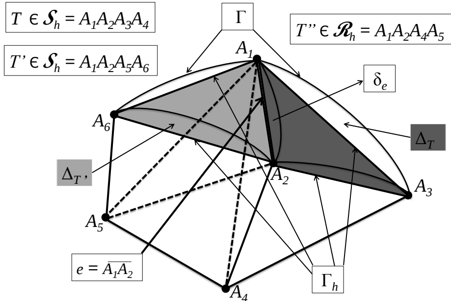
Figure 3: Sets \Delta_T , \Delta_{T'} , \delta_e for tetrahedra T, T' \in \mathcal{S}_h with a common edge e and a tetrahedron T'' \in \mathcal{R}_h
