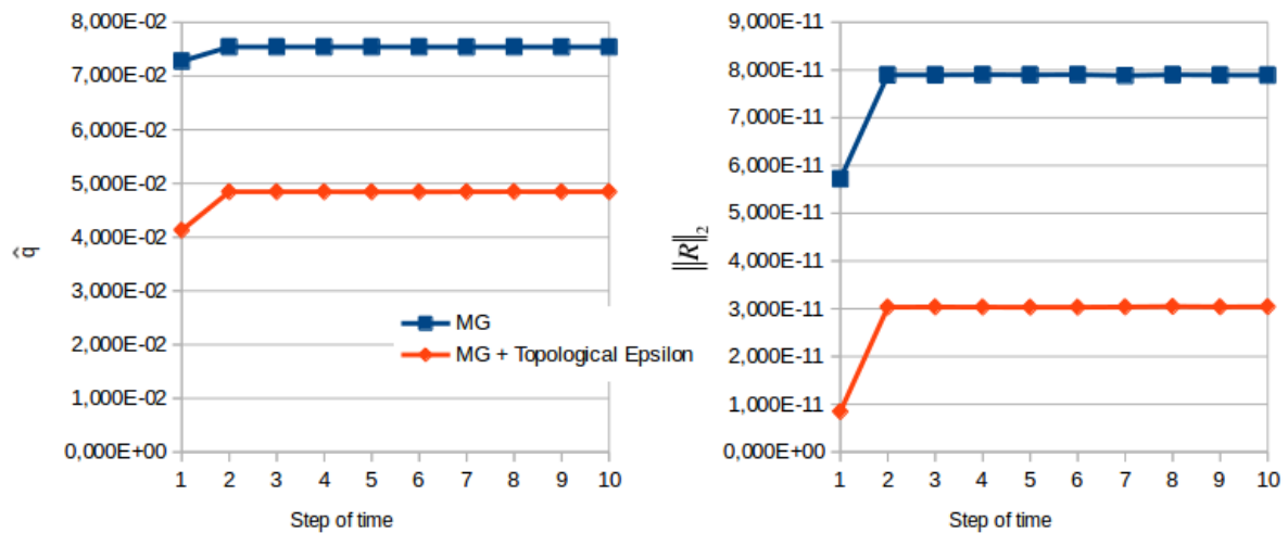
Figure 7: \hat{q}^{(k)} and \|R\|_2 at each instant of time
