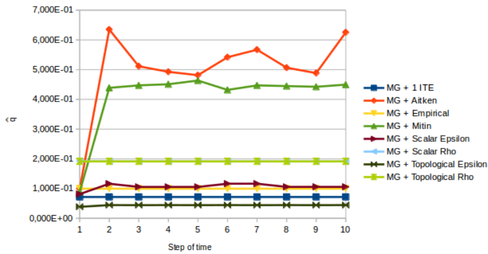
Figure 5: The mean empirical convergence factor for each step of time
