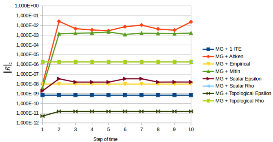
Figure 6: \|R\|_2 for each step of time
