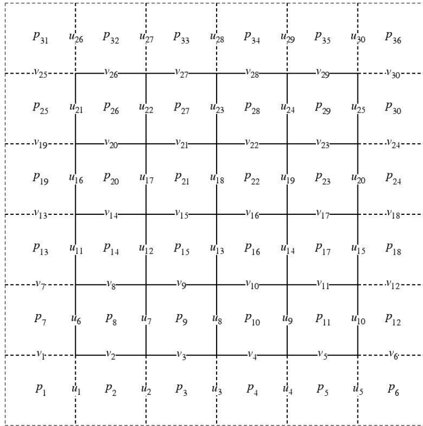
Figure 1: Lexicographical ordering
