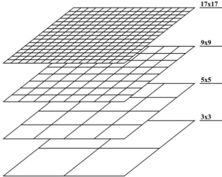
Figure 2: Meshes generation process (adapted from http://www.mgnet.org/mgnet/tutorials/xwb/mg.html )
