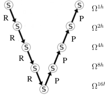
Figure 4: One cycle V Diagram applied in 5 meshes. S = smoothing, R = restriction, P = prolongation (Neundorff, 2016).
