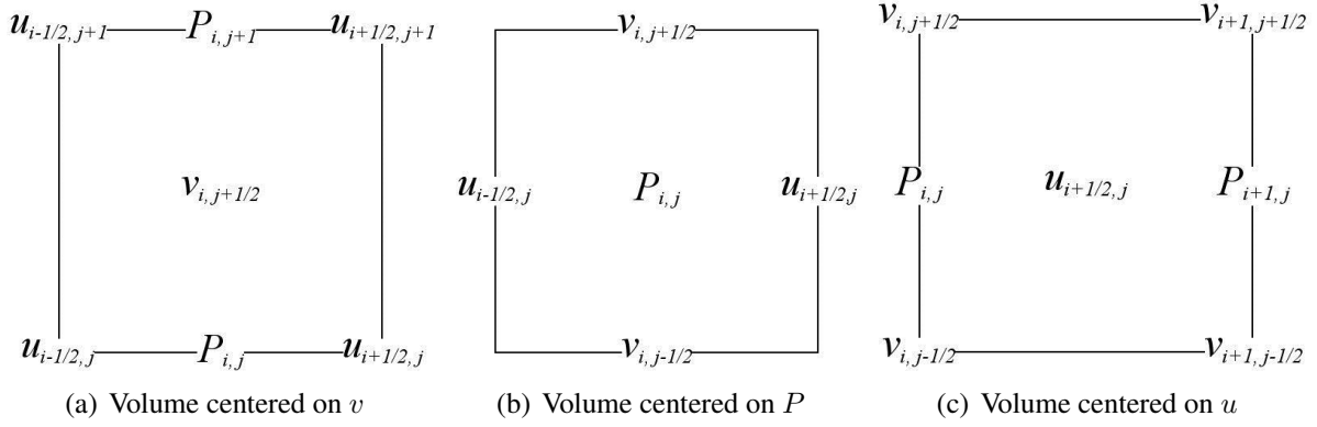
Figure 3: Control Volumes
