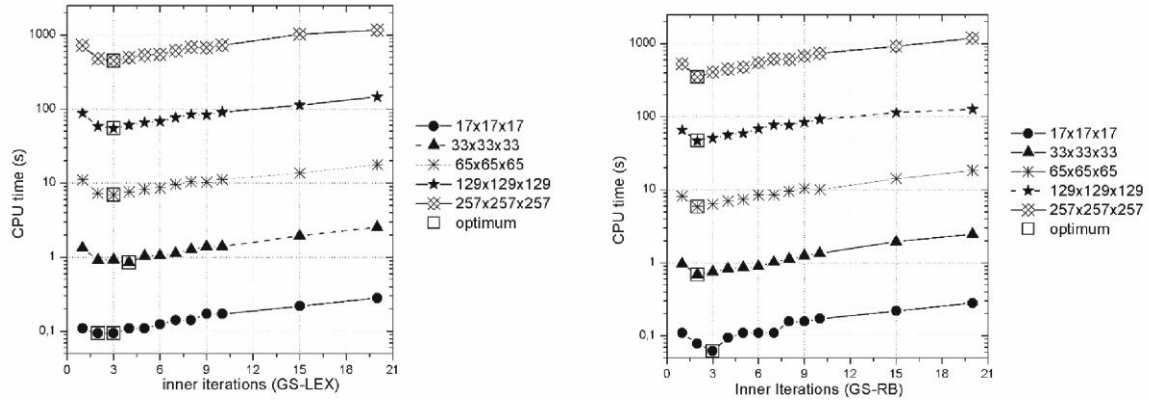
Figure 1: Analysis of number of smoothing for (a) lexicographical Gauss-Seidel and (b) red-black Gauss-Seidel, both using full weighting restriction
