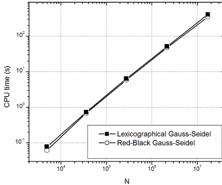
Figure 3: Comparison between lexicographical Gauss-Seidel (injection restriction) and Red-Black Gauss-Seidel (full weighting restriction)
