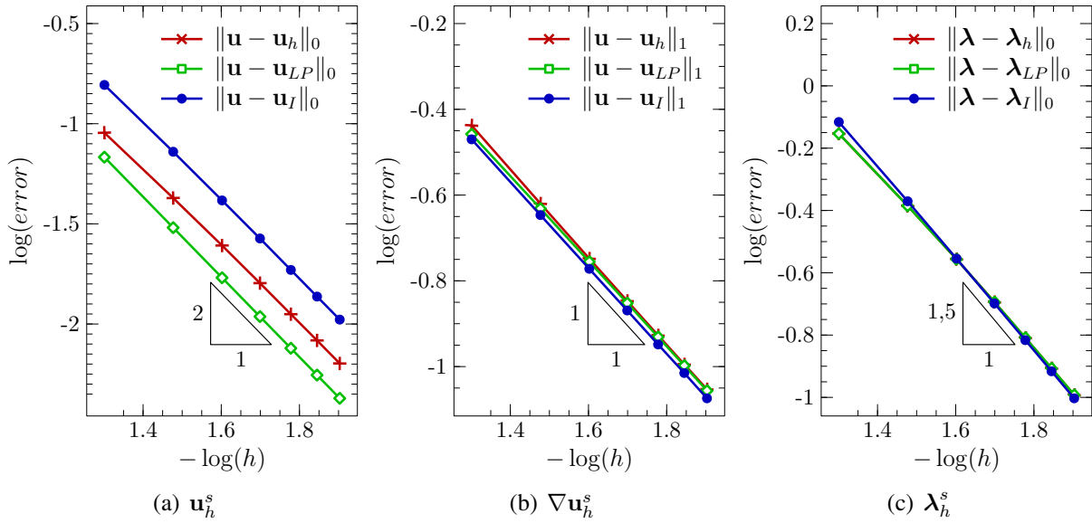
Figure 5: Elastic Wave: h -Convergence for the \mathbf{u}_h^s , \nabla \mathbf{u}_h^s and \lambda_h^s approximations by the SHEW hybrid method ( h ), Local Projection ( LP ) and Interpolant ( I ). Error in the L^2 -norm (left and right) and H^1 -seminorm for quadrilaterals elements \mathbb{Q}_1 - p_1 .
