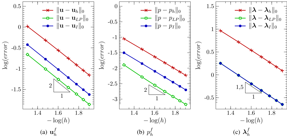
Figure 2: Helmholtz: h -Convergence for the \mathbf{u}_h^f , p_h^f and \lambda_h^f approximations by the SHHel hybrid method ( h ), Local Projection ( LP ) and Interpolant ( I ). Error in the L^2 -norm for quadrilaterals elements \mathbb{Q}_1\mathbb{Q}_1 - p_1 .
