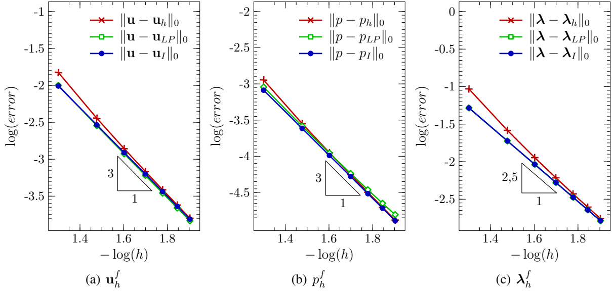
Figure 3: Helmholtz: h -Convergence for the u_h^f , p_h^f and \lambda_h^f approximations by the SHHel hybrid method ( h ), Local Projection (LP) and Interpolant (I). Error in the L^2 -norm for quadrilaterals elements \mathbb{Q}_2\mathbb{Q}_2 - p_2 .
