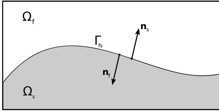
Figure 1: A sketch of the domain for the fluid-structure problem showing the interface of discontinuity.
