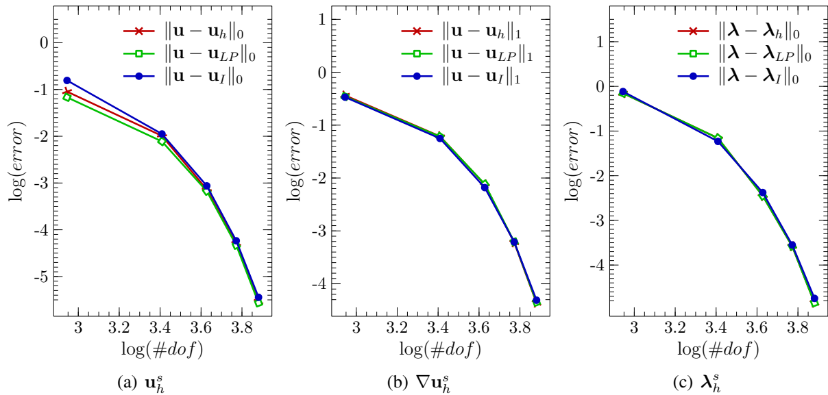
Figure 7: Elastic Wave: p -Convergence for the \mathbf{u}_h^s , \nabla \mathbf{u}_h^s and \lambda_h^s approximations by the SHEW hybrid method ( h ), Local Projection (LP) and Interpolant (I). Error in the L^2 -norm (left and right) and H^1 -seminorm for fixed 20 \times 20 elements mesh.
