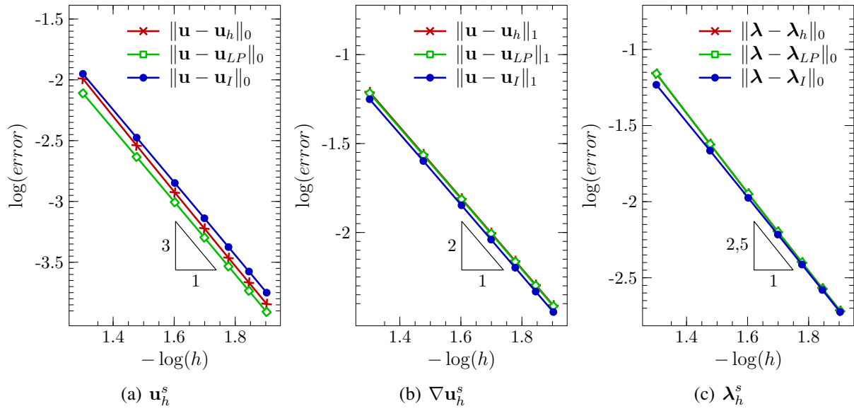
Figure 6: Elastic Wave: h -Convergence for the \mathbf{u}_h^s , \nabla \mathbf{u}_h^s and \lambda_h^s approximations by the SHEW hybrid method ( h ), Local Projection (LP) and Interpolant (I). Error in the L^2 -norm (left and right) and H^1 -seminorm for quadrilaterals elements \mathbb{Q}_2 - p_2 .
