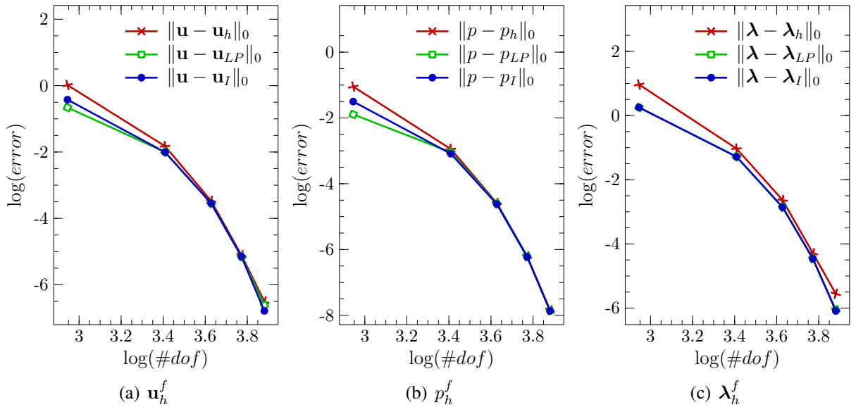
Figure 4: Helmholtz: p -Convergence for the u_h^f , p_h^f and \lambda_h^f approximations by the SHHel hybrid method ( h ), Local Projection (LP) and Interpolant (I). Error in the L^2 -norm for fixed 20 \times 20 elements mesh.
