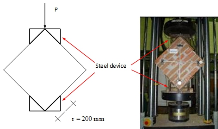
Figure 3: Diagonal compression test setup and measurement devices arrangement.
