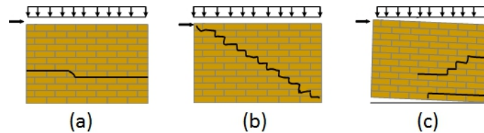
Figure 1: Modes of failure in URM walls subjected to in-plane forces: (a) Sliding along the bed joint. (b) Diagonal tension cracking. (c) Shear compression failure.
