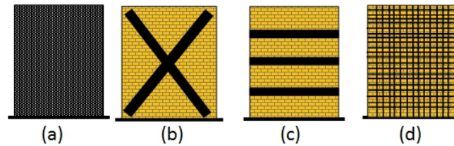
Figure 2: URM in plane FRP retrofitting schemes (a). Composite sheets bonded to entire wall surface. (b) Cross arrangements of FRP plates or laminates. (c) Horizontal strips of FRP laminates. (d) grid disposition of FRP.
